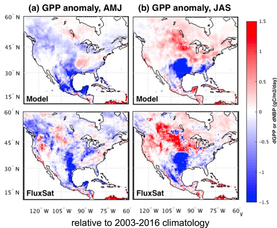
Lee et al. (2020) JGR-bio
