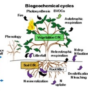
Carbon cycle
