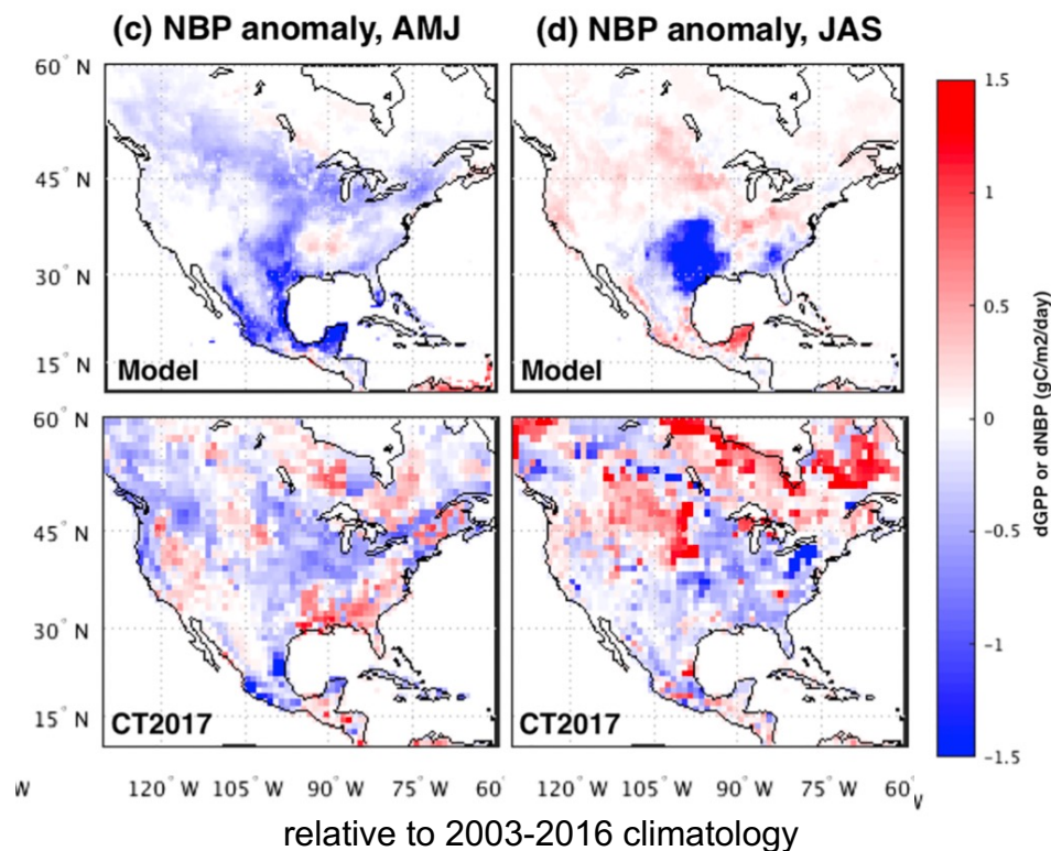
Anomaly for 2011 TexMex drought
