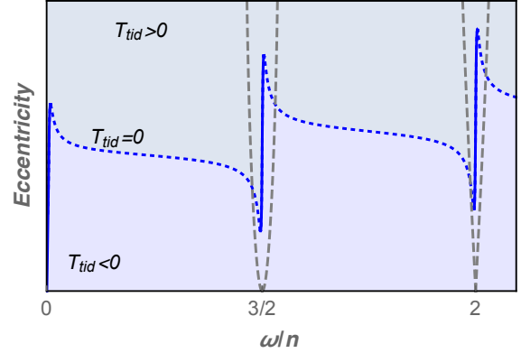
Fig. 5. Sketch of the equilibrium eccentricity, when the tidal torque vanishes, as a function of planetary rotation rate (blue curve). Solid portions of the curve near resonances depict stable equilibria, whereas dotted portions show unstable ones. Areas of positive torque are in gray, and of negative torque in blue. Dashed gray curves show the area covered by librations inside the resonances, that is, the resonance width (see Eq. (7)). With realistic values for the triaxiality and the Maxwell time, both the kink around the resonances and the resonance width would be much narrower and difficult to see.
