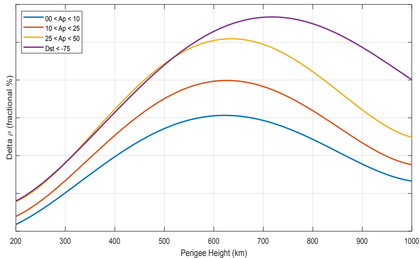
Figure N-9 Behavior of Relative Density Error by Perigee Height and Solar Activity
