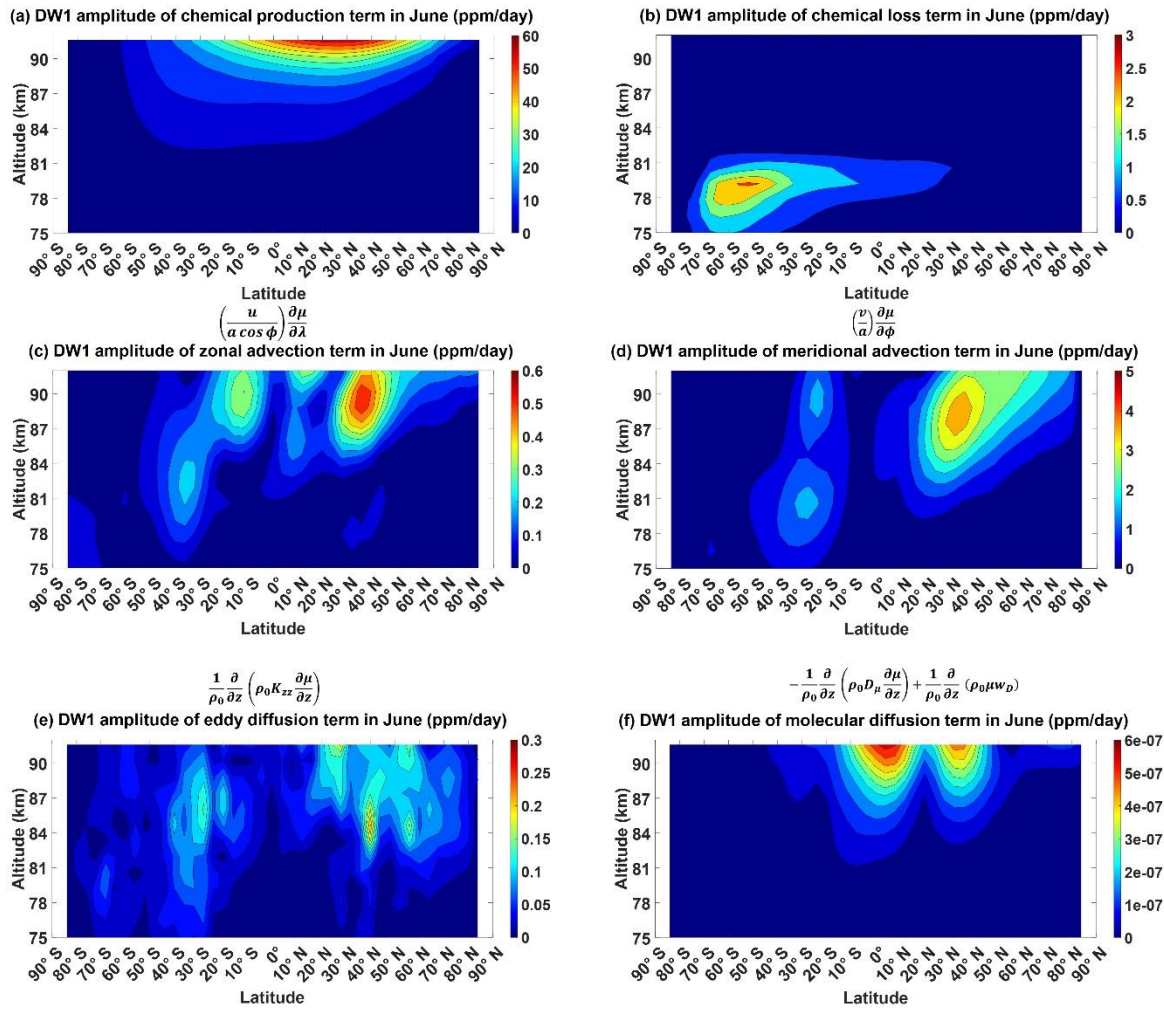
650 Figure B2: Migrating Diurnal Tide component in June solstice of (a) CO's chemical production term, (b) CO's chemical loss term, (c) CO's zonal advection term, (d) CO's meridional advection term, (e) CO's eddy diffusion term and (f) CO's molecular diffusion term. All are in units of ppm/day.
