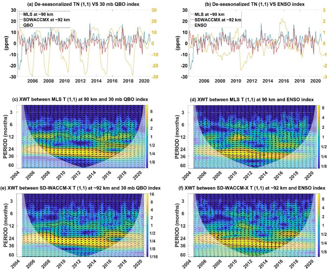
665 Figure C1: (a) De-seasonalized time-series of MLS temperature (1,1) at ~90 km, SD-WACCM-X temperature (1,1) at ~92 km and the QBO index. (b) De-seasonalized time-series of MLS temperature (1,1) at ~90 km, SD-WACCM-X temperature (1,1) at ~92 km and the ENSO index. (c) Cross-wavelet spectrum between MLS temperature (1,1) at ~90 km and the QBO index. (d) Cross-wavelet spectrum between MLS temperature (1,1) at ~90 km and the ENSO index. (e) Cross-wavelet spectrum between SD-WACCM-X temperature (1,1) at ~92 km and the QBO index. (f) Cross-wavelet spectrum between SD-WACCM-X temperature (1,1) at ~92 km and the ENSO index.
