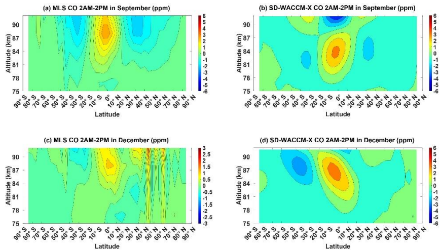
615 Figure A2: Migrating Diurnal Tide component of (a) MLS CO in September equinox, (b) SD-WACCM-X CO in September equinox, (c) MLS CO in December solstice and (d) SD-WACCM-X CO in December solstice. All are in units of ppm.
