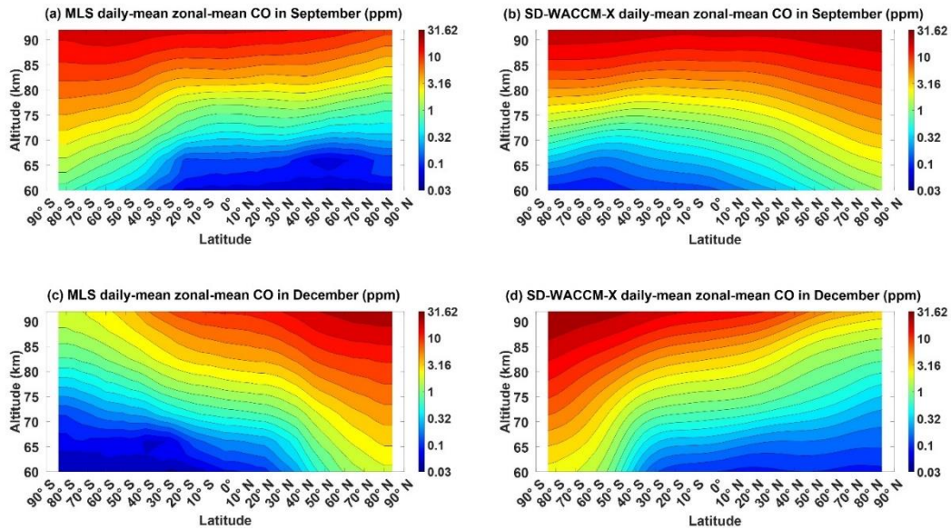
610 Figure A1: Daily-mean zonal-mean component of (a) MLS CO in September equinox, (b) SD-WACCM-X CO in September equinox, (c) MLS CO in December solstice and (d) SD-WACCM-X CO in December solstice. All are in units of ppm.
