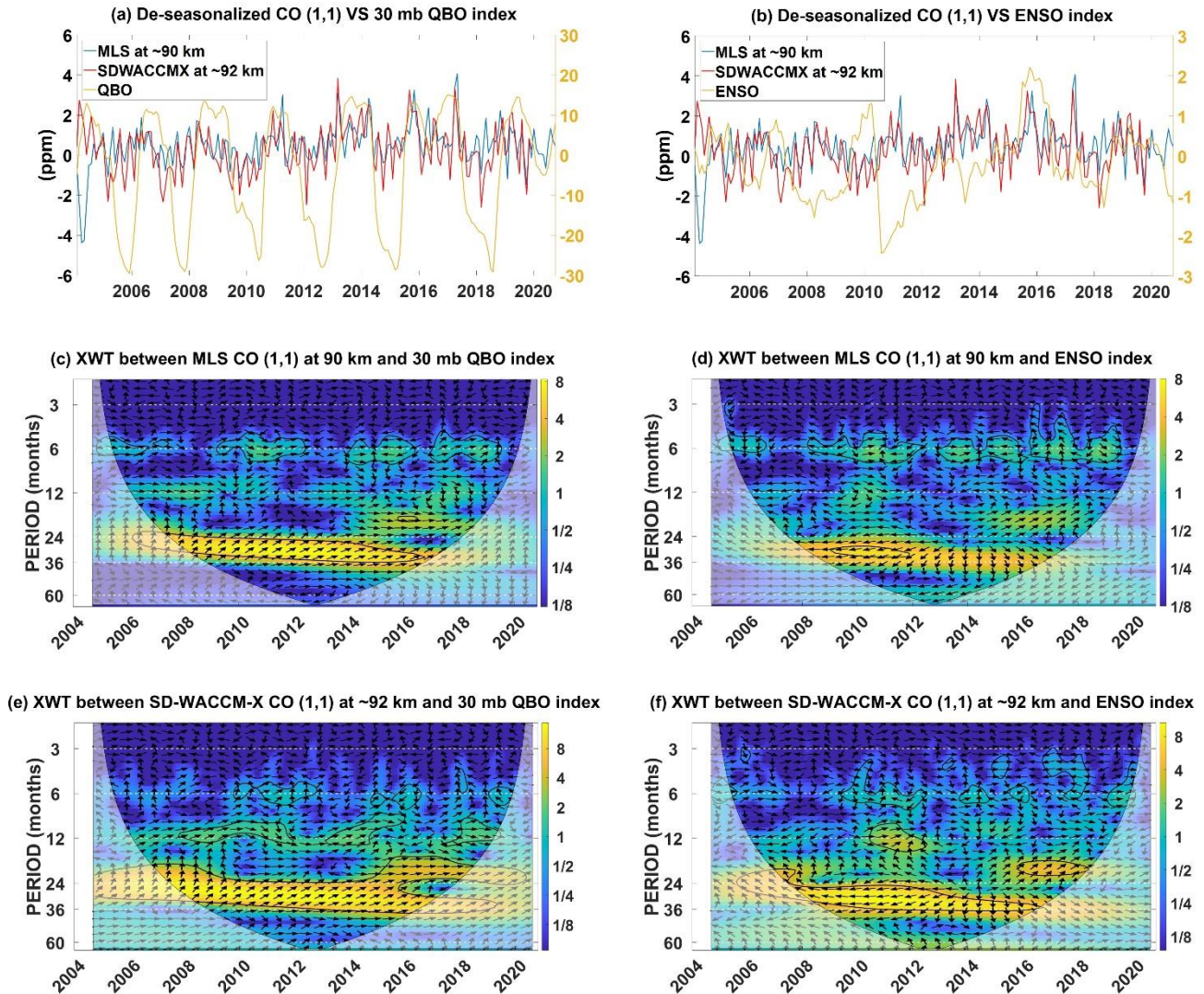
440 Figure 9: (a) De-seasonalized time-series of MLS CO (1,1) at ~90 km, SD-WACCM-X CO (1,1) at ~92 km and the QBO index. (b) De-seasonalized time-series of MLS CO (1,1) at ~90 km, SD-WACCM-X CO (1,1) at ~92 km and the ENSO index. (c) Cross-wavelet (XWT) spectrum between MLS CO (1,1) at ~90 km and the QBO index. (d) Cross-wavelet spectrum between MLS CO (1,1) at ~90 km and the ENSO index. (e) Cross-wavelet spectrum between SD-WACCM-X CO (1,1) at ~92 km and the QBO index. (f) Cross-wavelet spectrum between SD-WACCM-X CO (1,1) at ~92 km and the ENSO index.
