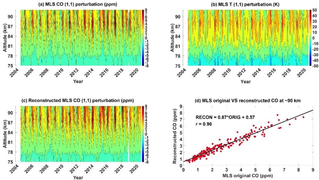
Figure 7: (1,1) component of (a) MLS CO, (b) MLS temperature and (c) MLS CO reconstructed using the adiabatic displacement method from 2004 till 2021. (d) Scatter plot between MLS CO's (1,1) component at ~90 km and that reconstructed using the adiabatic displacement method. Units are specified in the plots.
