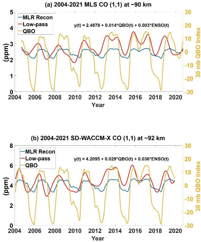
530 Figure 10: (a) MLS CO (1,1) at ~90 km reconstructed using multiple linear projection (MLR), low pass filtered and the 30 mb QBO index from 2004 till 2020. (b) Same as (a) but for SD-WACCM-X CO (1,1) at ~92 km. Equations within the subplots are the MLR fits.
