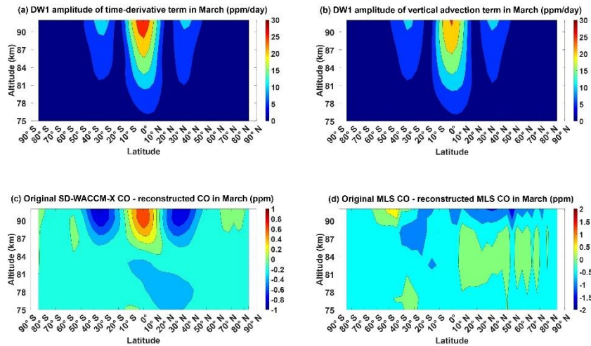
275 Figure 4: Migrating Diurnal Tide component in March equinox of (a) CO's time-derivative term and (b) CO's vertical advection term. (c) Difference between SD-WACCM-X CO's DW1 component and SD-WACCM-X CO's DW1 component reconstructed using adiabatic displacement method. (d) Difference between MLS CO's DW1 component and MLS CO's DW1 component reconstructed using adiabatic displacement method. Units are specified in the plots.
