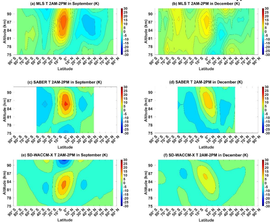
620 Figure A3: Migrating Diurnal Tide component of (a) MLS temperature in September equinox, (b) MLS temperature in December solstice, (c) SABER temperature in September equinox, (d) SABER temperature in December solstice, (e) SD-WACCM-X temperature in September equinox and (f) SD-WACCM-X temperature in December solstice. All are in units of K.
