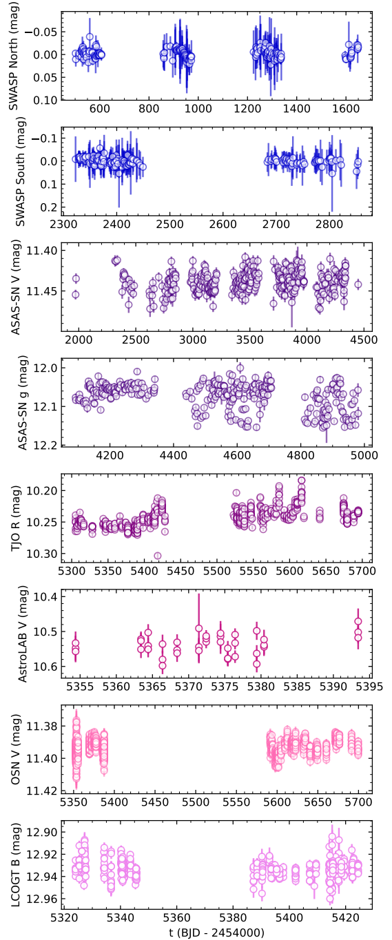
Fig. 3. Used photometric variability sets (Sect. 3.5). From top to bottom: SuperWASP (North and South), ASAS-SN ( V and g' ), TJO ( R ), AstroLAB ( V ), OSN ( V ), and LCOGT ( B ). For homogeneity, we transformed TJO, OSN, and LCOGT (normalised) fluxes to differential magnitudes.
