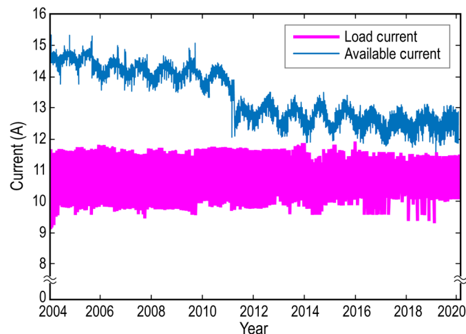
Fig. 10 Average solar panel-generated current over time for the entire Spitzer mission.
