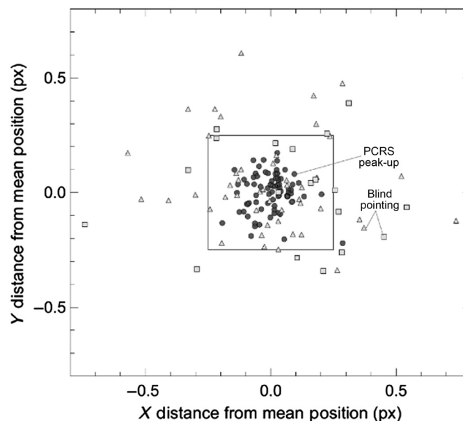
Fig. 11 Comparison of pointing repeatability using peak-up versus blind pointing. Each point represents the mean centroid of the first 64 frames of the following: 78 observations (dark circles) beginning with PCRS peak-up followed by an offset to the 4.5\text{-}\mu\text{m} sweet-spot using gyros; 20 observations (light squares) using PCRS peak-up and the star tracker for the offset; and 48 observations (light triangles) initiated without PCRS peak-up. Each set of symbols has had the mean position of the set subtracted. A 0.5 \times 0.5 pixel square is overlaid on the plot, indicating the size of the sweet-spot region. 28
