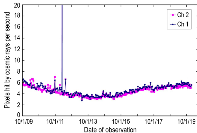
Fig. 8 Average number of pixels in the IRAC arrays affected by cosmic rays in the calibration frames taken during the Spitzer warm mission. 3 The array formats were 256 \times 256 30\text{-}\mu\text{m} -squared pixels. The spike in 2012 was due to a solar flare.
