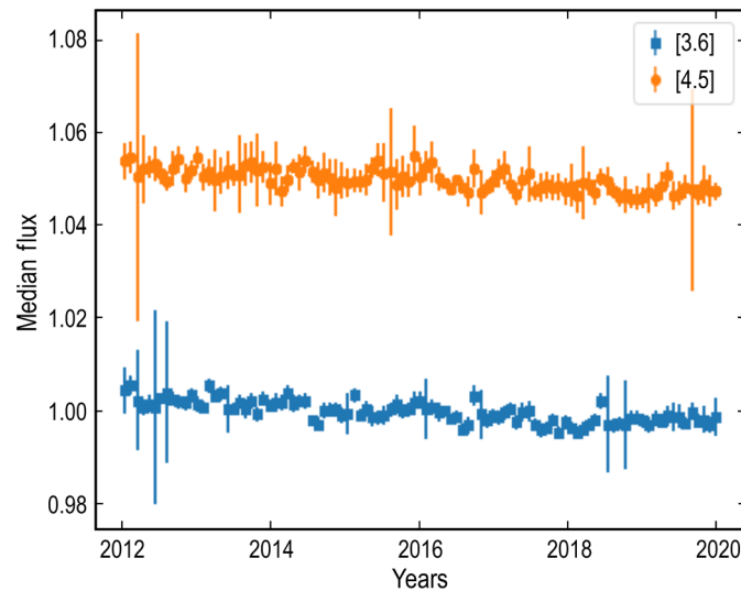
Fig. 9 Average IRAC responsivity versus time for the final 8 years of the warm mission, based on the measured flux from seven primary calibrator stars. The seven primary calibrators for Spitzer were KF09T1, KF06T2, KF08T3, KF06T1, NPM1p67, NPM1p60, and 1812095. 23
