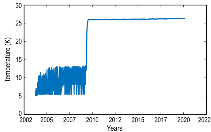
Fig. 6 Spitzer primary mirror temperature versus time over the entire Spitzer mission. The fluctuations in temperature seen prior to the start of the warm mission in mid-2009 reflect the helium utilization strategy described in the text.
