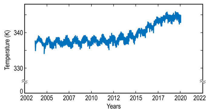
Fig. 4 The average temperature of the lower, solar cell-containing portion of the solar panel versus time over the entire Spitzer mission. The annual periodicity seen in this and the other temperature data reflects the eccentricity of Spitzer's orbit.
