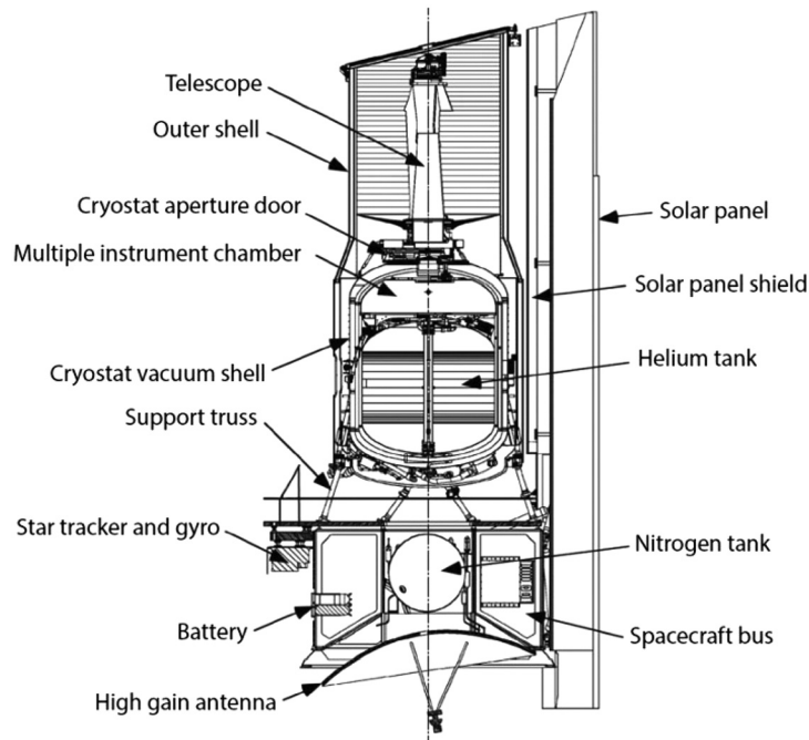
Fig. 1 Cutaway view of the Spitzer observatory. 2 The dust cover atop the telescope tube was jettisoned a few days after launch, and the cryostat aperture door was opened shortly afterward to admit infrared radiation into the instrument chamber. See papers listed in the Appendix for a detailed discussion of the in-orbit checkout for Spitzer .
