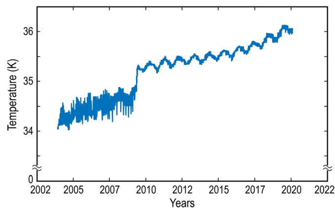
Fig. 5 Spitzer outer shell temperature versus time over the entire Spitzer mission. The discontinuity in 2009 reflects the exhaustion of the liquid helium and the start of the warm mission, when vapor cooling was no longer available. The oscillations in temperature seen before this reflects the variation in vapor cooling resulting from the helium utilization strategy described in the text.
