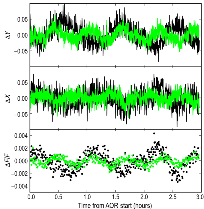
Fig. 12 Effects of tightening battery heater dead band on pointing and photometric stability. The upper two panels show the variation of the (x, y) position of the centroided stellar image on the array, and the lower panel shows the variation in measured signal, all as a function of time. Black points are data taken before the dead band was tightened; green points were taken after the adjustment.
