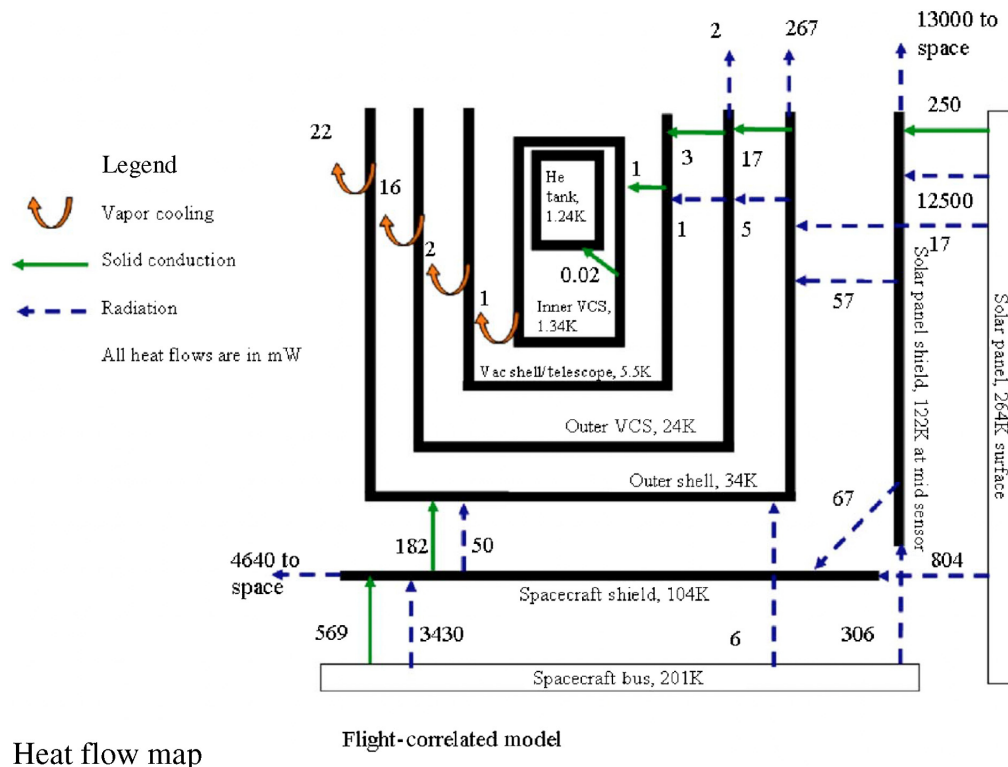
Fig. 2 Ball Aerospace thermal model. 1 Heat input is solely from insolation on the solar panel. Cooling of the cryogenic telescope assembly is accomplished by radiation and vapor cooling. Heat is transferred through the system along the paths indicated by the arrows by radiation (dashed blue arrows), conduction (solid green arrows), and vapor cooling (broad orange arrows). The equilibrium temperatures for the various observatory components are given for the case when the cryogenic telescope is operating at 5.5 K. The model assumes a focal-plane heat dissipation of 4 mW and an insolation of 5.3 kW. Courtesy of Ball Aerospace/JPL-Caltech.
