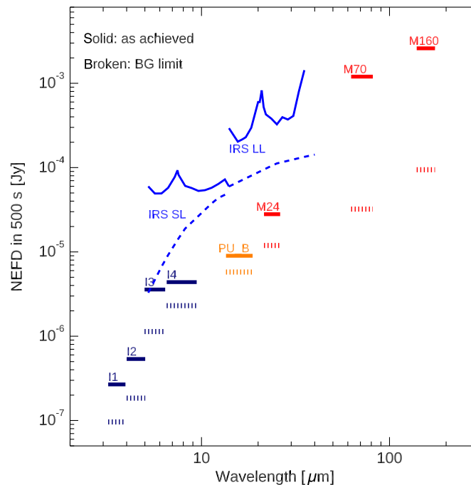
Fig. 7 Achieved Spitzer point source sensitivities (solid lines, 1\sigma in 500 s) 2 compared with estimates of fundamental limits imposed by the zodiacal background. The short vertical lines under each instrumental bandpass show the zodiacal background-limited NEFD estimate for the bandpass, assuming noise from the zodiacal light in an annual average sightline viewing the north ecliptic pole. Note that the achieved performance is closest to the background limit in the 8 to 24 \mu\text{m} range where the background is at its brightest. The background couples in both polarizations with a square bandpass of the plotted width and total transmission (including detector absorption efficiency) of 0.44, 0.42, 0.14, and 0.30 for IRAC bands 3.6, 4.5, 5.8, and 8.0 \mu\text{m} , respectively, 0.6, 0.18, and 0.15 for MIPS 24, 70, and 160 \mu\text{m} , respectively, and 0.65 for the IRS blue peak-up array (PU B) at 16 \mu\text{m} . Perfect detectors that add no noise other than generation-recombination noise are assumed throughout. The sensitivity achieved by MIPS is degraded below the zodiacal limit, in part, by the effects of confusion at both 70 and 160 \mu\text{m} ; it is appreciable in both channels in 500 s. The IRS short-low and long-low module sensitivities are referred to a \lambda/\delta\lambda = 50 bin; the estimates adopt wavelength-independent efficiencies of 12% and 8.5%, respectively; this is meant to include all sources of loss including slit coupling, blaze efficiency in both polarizations, filters, and detector quantum efficiency. For all, it is assumed that the 14% obscured 85-cm Spitzer telescope ( A_{\text{geom}} = 0.489 \text{ m}^2 ) couples to a point source with 75% aperture efficiency. The \sqrt{2} photoelectron recombination penalty is included for all bands except IRAC 1 and 2, where it does not apply.
