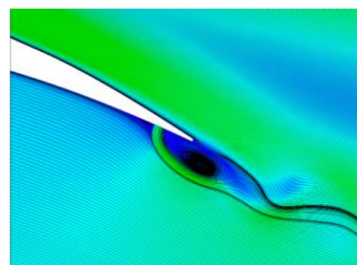
Pressure side microjet
