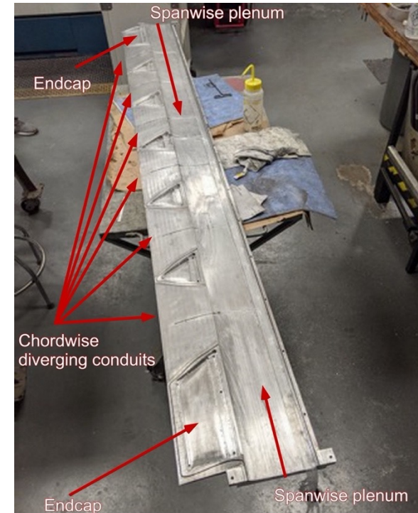
Flap lower-side panel depicting microjet flow paths
