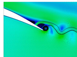
Suction side microjet
