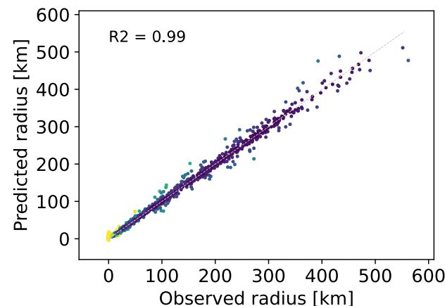
5. Neural network
