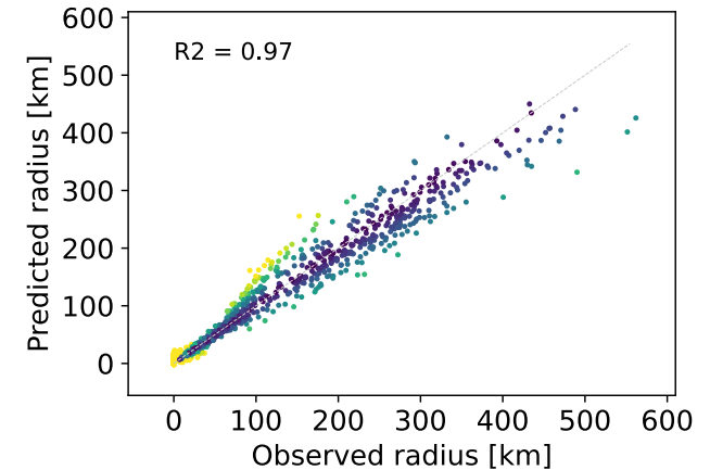
5. Neural network
