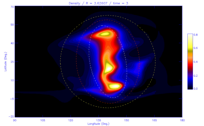
Fig. 9. Figure showing the MHD scaled density at R = 3.62 R_{\odot} spherical slice in longitude and latitude at the same time step of the simulated white-light data ( t = 3 code time units). R = 3.62 R_{\odot} is the slice at which the CME cross-section had the largest extent in both latitude and longitude. The medium red ellipse overlay was used to derive the ground truth for the CME parameters of longitude, latitude, tilt, half-angle and ratio, and the white ellipses were used as the uncertainty.
