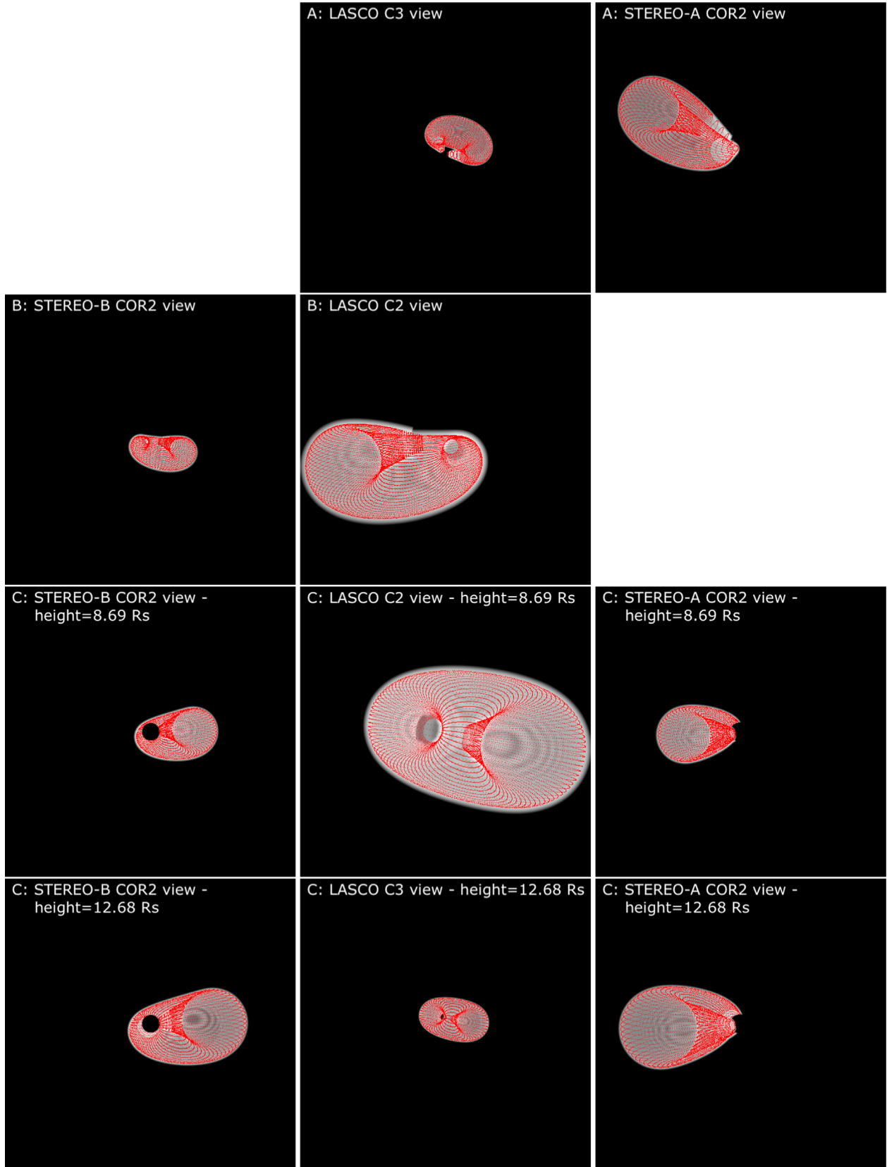
Fig. 2. Images of synthetic white-light data generated by GCS ray-tracing for configurations A (top row), B (second row), and C (bottom two rows), with STEREO-B (left), LASCO (middle), and STEREO-A (right) views. For configuration C, synthetic images were created for two different heights of 8.69 and 12.68 R_{\odot} . The true GCS fits used to create these synthetic data, are shown as the red wire frame with the parameters given in Table 1. A schematic of the configurations is provided in Fig. 1.
