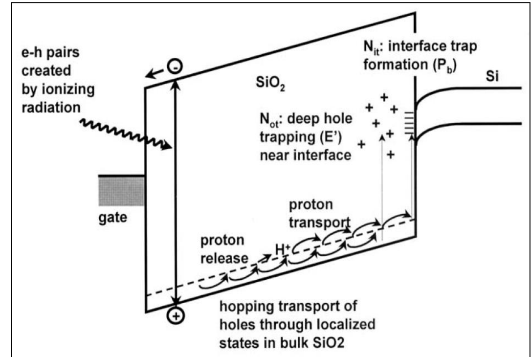
Processes Involved in TID Damage
