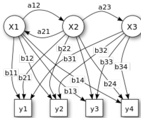
Figure 29. Probabilistic parameters of a Hidden Markov
