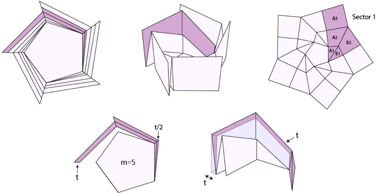
Fig. 3. The m5_h2_r1 pattern is illustrated in stowed and deployed configurations. Top from left: The pattern's top view is shown. An isometric view of the paper-thin pattern is illustrated stowed. The flasher is deployed with one of five sectors highlighted and its panels labeled. On the bottom row, one sector of the five-sided pattern is featured to clarify how it stows with thickness added.
