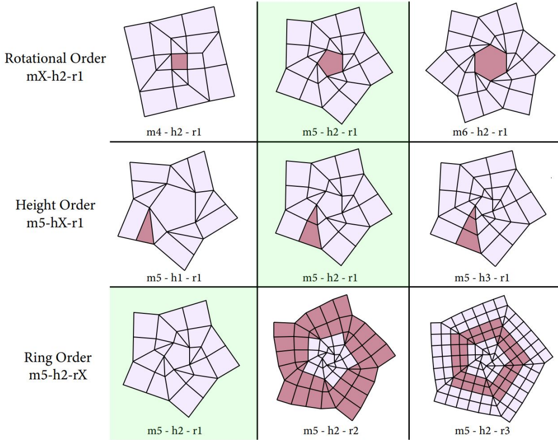
Fig. 2. Several candidate origami flasher patterns with varying rotational, height, and ring orders are depicted. The pattern shaded in green, m5-h2-r1, was selected as the pattern for our deployable space array. Note that a standard dr value of 1.6 was used to generate the above patterns. The m5-h2-r3 pattern is an exception with a dr of 0.
