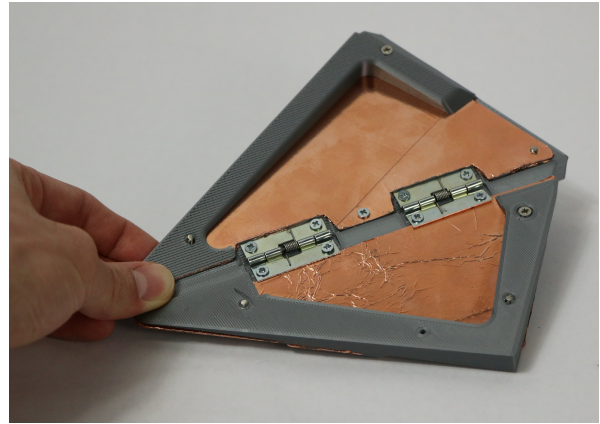
Fig. 8. Panels A1 and B1 are connected via two spring hinges. The copper portions replace the green region in Figure 7. The copper panels lie coplanar to each other when deployed.
