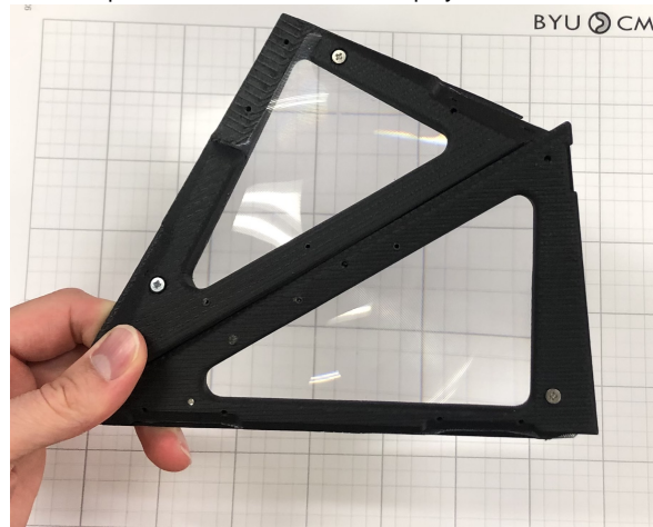
Fig. 9. A fresnel lens is secured within the frames of panels A1 and B1.
