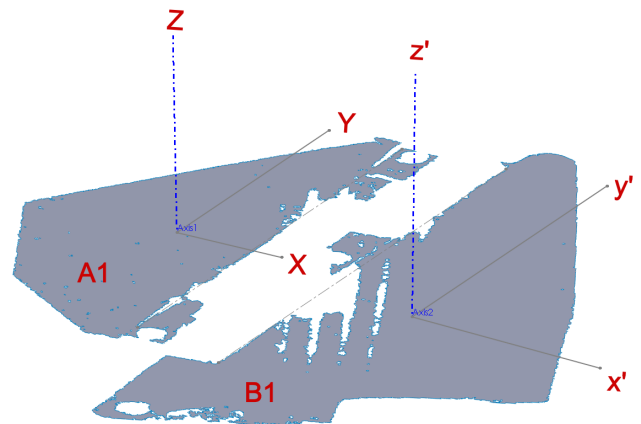
Fig. 6. The surfaces and coordinate systems of panels A1 and B1, as measured using a red-laser 3D scanner, used to determine the relative misalignment are depicted.
