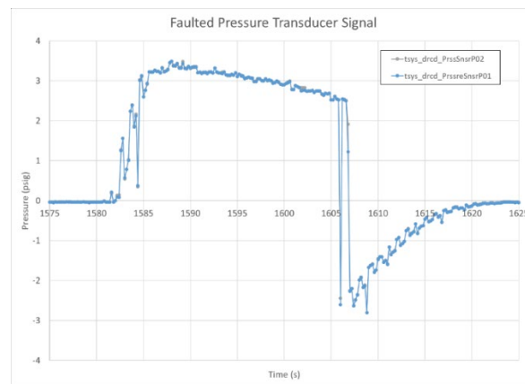
Figure 3. Pressure Transducer data plot showing Toilet Fault condition. The separator pressure inverted to a negative reading for ~17 seconds during shutdown.
