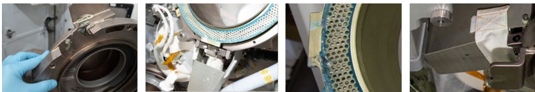
Figure 4. Dried residue from pretreat and water solution release on UWMS (left to right) A.) commode cover, B.) uncovered but installed TAF and filter access door, C.) removed TAF, and D.) the hose cover adjacent to the air outlet.
