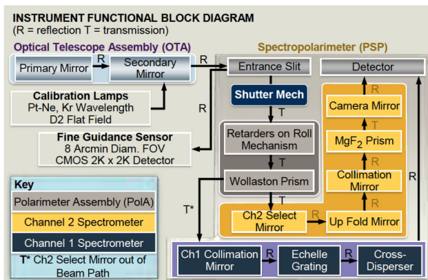
Fig. 13 Polstar Instrument Block Diagram. The OTA collects light with a symmetric optical design that minimized instrumental polarization and delivers that light to the entrance slit. Calibration lamps are mounted in the secondary shadow to feed the optical instrument. A mechanical shutter controls light entering the instrument, and the slit has a silvered back to allow the field to be used for guidance via the FGS. The light passes through a rotating modulator and is split by the prism to deliver a two-beam optical encoding of the polarimetric signal, which is then dispersed by either channel and recorded at the detector
