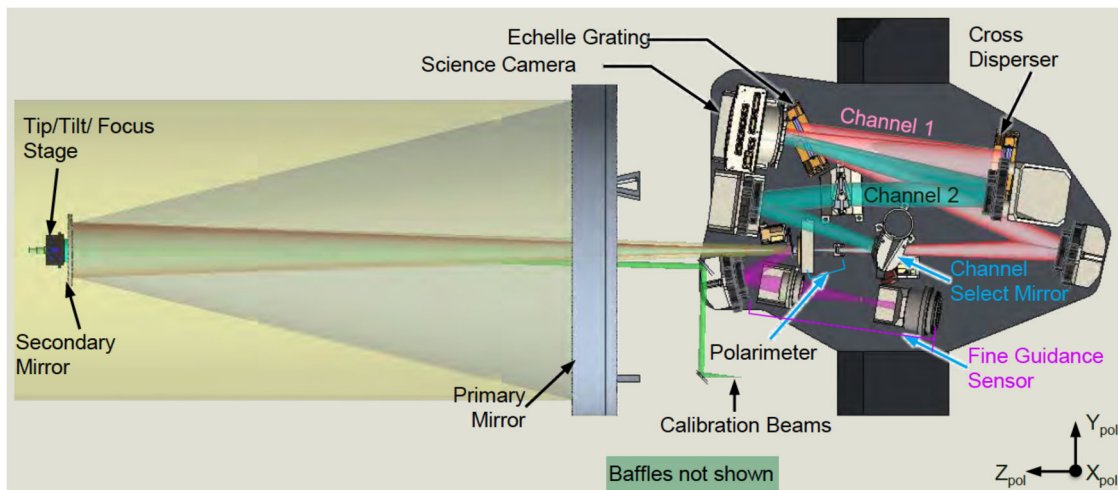
Fig. 12 Polstar Instrument Design. The opto-mechanical design uses an ultra-stable optical bench to provide a repeatable measurement from modulator position to modulator position, and is kinematically
