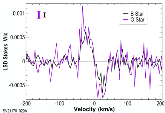
Fig. 4 UV Magnetometry. Modeled Stokes-V profiles from the LSD method for O and B stars with surface field of 3 kG for SNR=100 per resel, requiring resolution R=30k and LSD-improved polarization precision 2 \times 10^{-4} . Representative errors indicated at upper left
