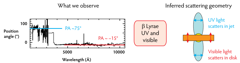
Fig. 6 Polarized spectrum (left) of \beta Lyr and interpretive picture (right), based on the study by Hoffman et al. (1998). The 90^\circ position angle flip between the near-UV and optical continuum provided key evidence for a jet or outflow in the system oriented orthogonal to the thick accretion disk
