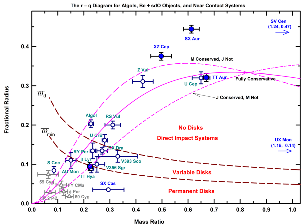
Fig. 1 The locations of targets selected for this study (cf. Sect. 3) in the r - q diagram. The near contact systems are plotted with solid blue circles, while the Algol binaries are indicated by open circles and cyan labels. The objects plotted with open gray triangles are Be+sdO systems. The error bars are from individual papers on each star. The magenta long-dashed and short-dashed curves indicate, respectively, trajectories of predominantly nonconserved angular momentum and nonconserved mass transfer, as discussed in the text. The evolutionary track for fully conservative mass transfer is shown by the solid magenta curve
