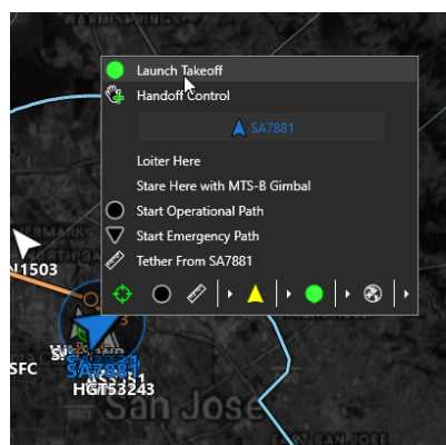
Fig. 3 Context menu used to manually send a takeoff command to a vehicle in the Voice condition.
