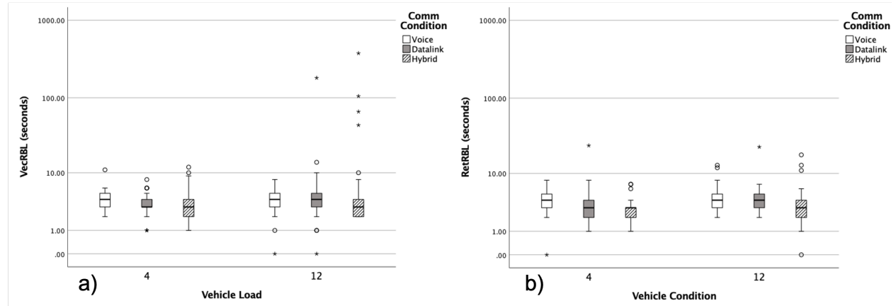
Fig. 13 Boxplots of VecRBL and RetRBL by condition. Outliers and extreme outliers identified by circles (○) and asterisks (*), respectively. Note that the vertical axes employ logarithmic scales.
