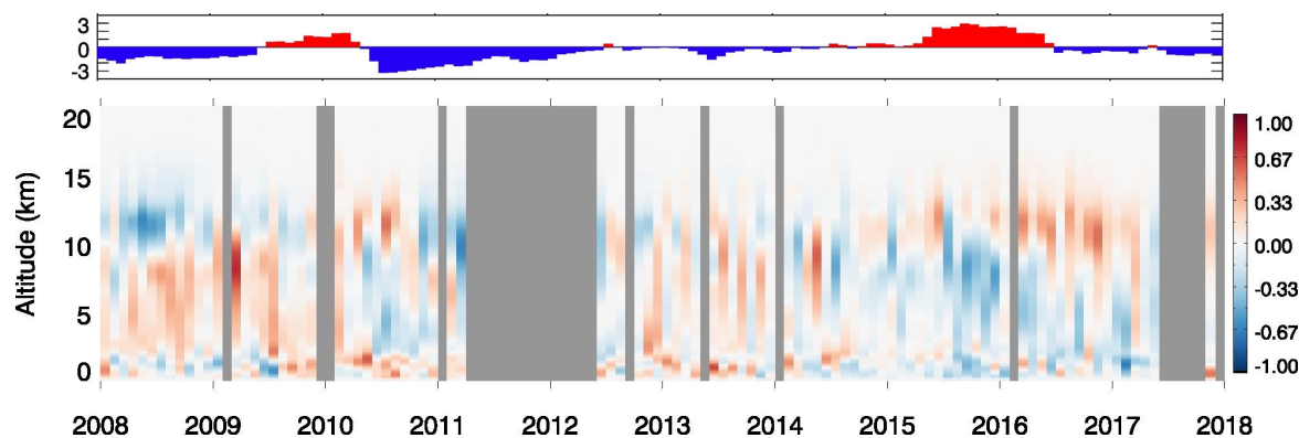
60°S-60°N Cloud Occurrence Anomaly (%)
