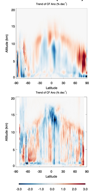
2008-2017 Cloud Trend (% dec -1 )
