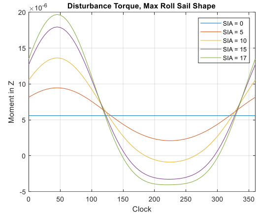
Fig 5. Maximum Roll Disturbance Torque
