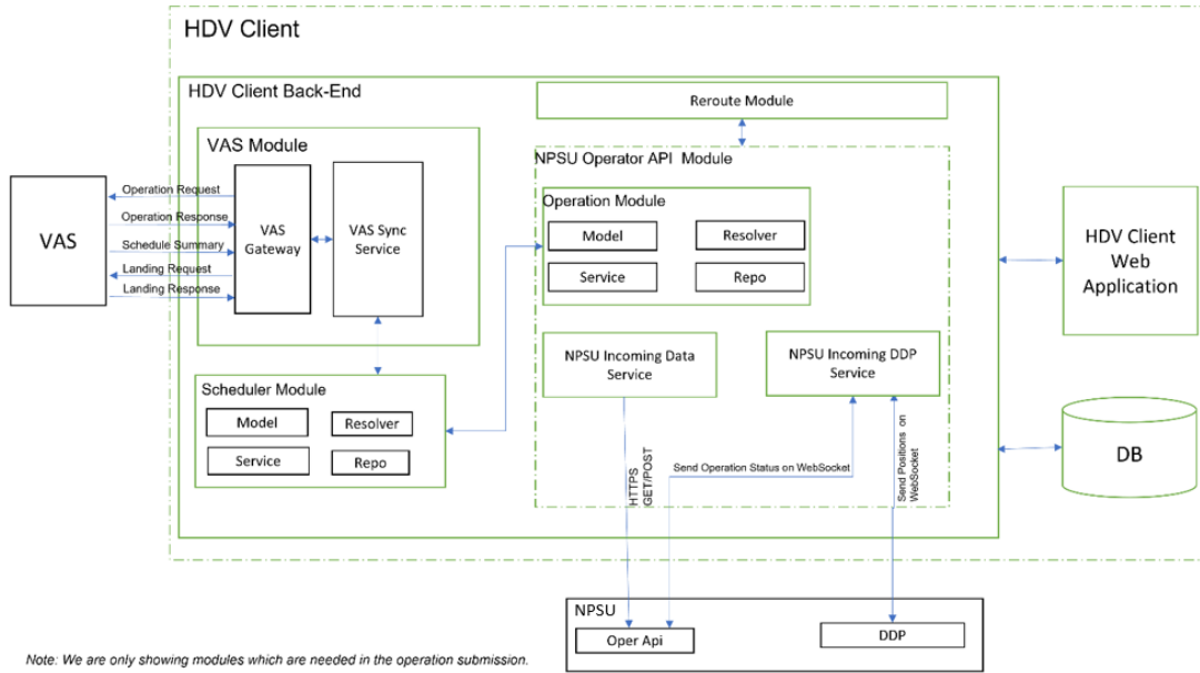
Fig. 5 A base nominal operation submission data flow.
