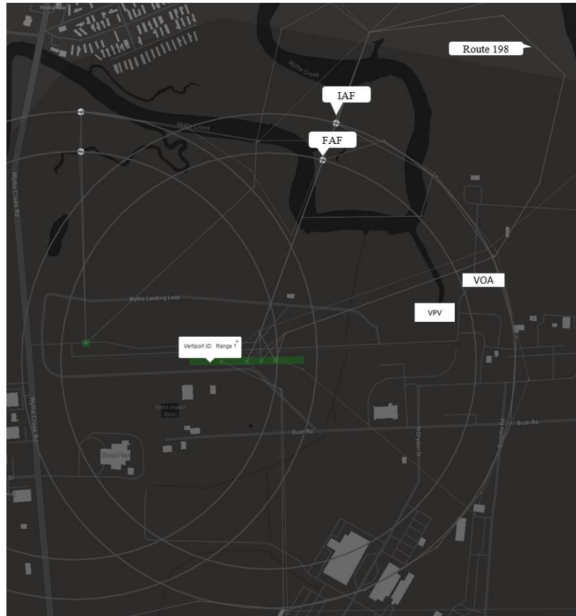
Fig. 19 Vertiport design with VOA/VPV rings, IAF, and FAF.
