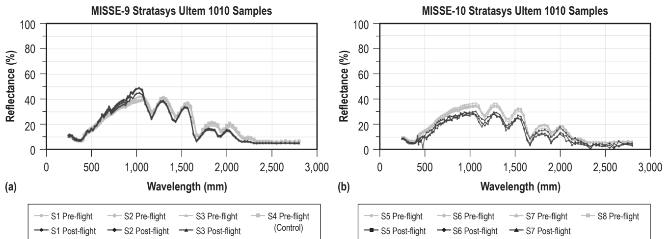
Figure 10. Reflectance data on Stratasys Ultem 1010 for (a) MISSE-9 and (b) MISSE-10.
