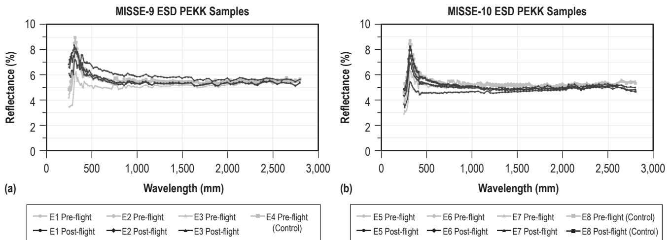
Figure 12. Reflectance data on Stratasy ESD PEKK for (a) MISSE-9 and (b) MISSE-10.
