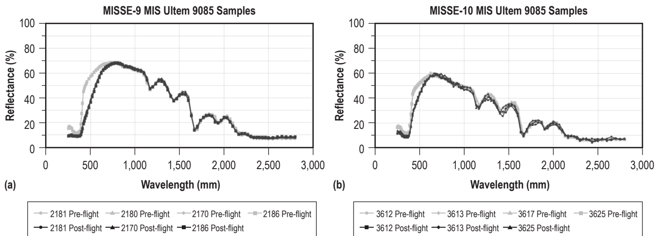
Figure 8. Reflectance data on MIS Ultem 9085 for (a) MISSE-9 and (b) MISSE-10.
