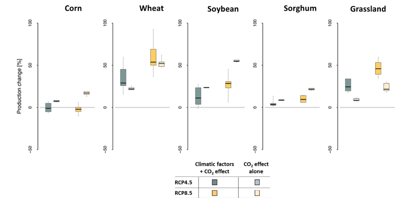
Fig. 2. U.S. crop production response from LPJmL showing the percent change between 1980-2005 and 2075-2100. RCP4.5 is shown in green and RCP8.5 in orange. The darker hues show the combined effects of climatic factors (precipitation and temperature) together with CO 2 fertilization. The lighter hues show the isolated effect of CO 2 fertilization. The boxplots show the distribution of effects across 6 CMIP5-LOCA climate models. The horizontal bars within the boxes indicate the median, the ends of the whiskers extend to 1.5 times the interquartile range.
