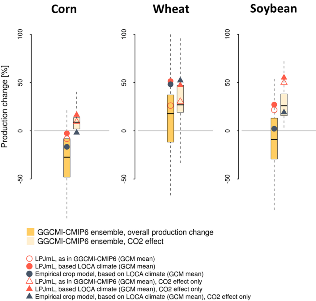
Fig. 3. U.S. crop production responses from the LPJmL and empirical crop models driven by downscaled CMIP5 climate simulations in comparison to the GGCM-IP6 ensemble, showing the percent change from 1980-2005 to 2075-2100. All climate model inputs for these simulations were from the RCP8.5 scenario. For each crop, the symbols on the left side show the overall production change, whereas the symbols on the right show the CO 2 effect alone. The orange box plots show the distribution of results from the GGCM ensemble, including 12 crop models driven by 5 CMIP6 climate models (Jägermeyr et al., 2021 for details). The horizontal bars within the boxes indicate the median across all climate-crop model combinations, the boxes show the interquartile range, and the whiskers extend to 1.5 times the interquartile range. The open red circles show the LPJmL response driven by the CMIP6 models used in the GGCM ensemble. The solid red circles show the LPJmL response driven by CMIP5-LOCA climate model inputs. The triangles show similar results but driven only by the CO 2 effect. The closed grey circles show the econometric model response driven by LOCA climate model inputs.
