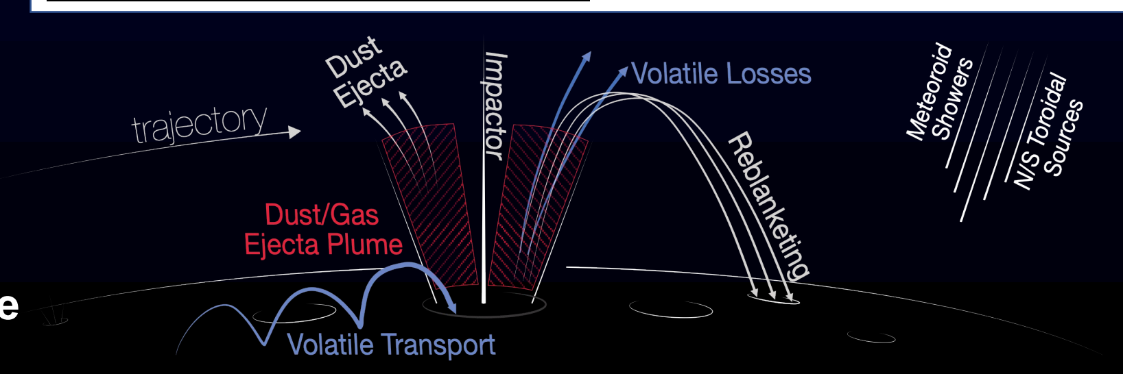
Figure 11. Meteoroid impacts implications for volatile and water cycles (Szalay).
