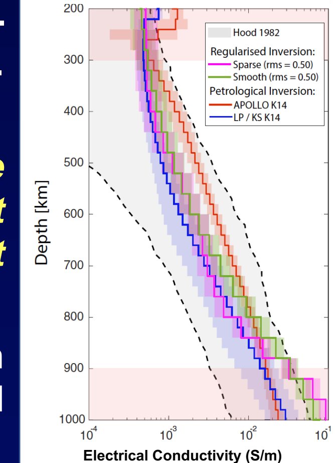
Figure 6. Conductivity profiles constrain composition (Mittelholz et al 2022, JGR Planets).
