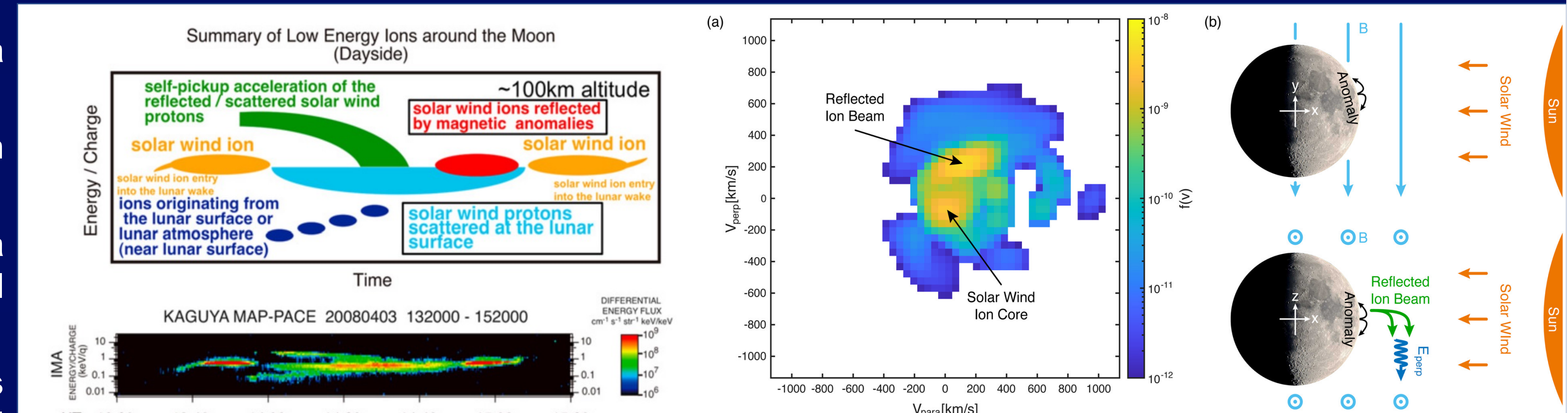
Figure 9. Example observed reflected ion beam (Chu et al. 2021, JGR Space Physics).
