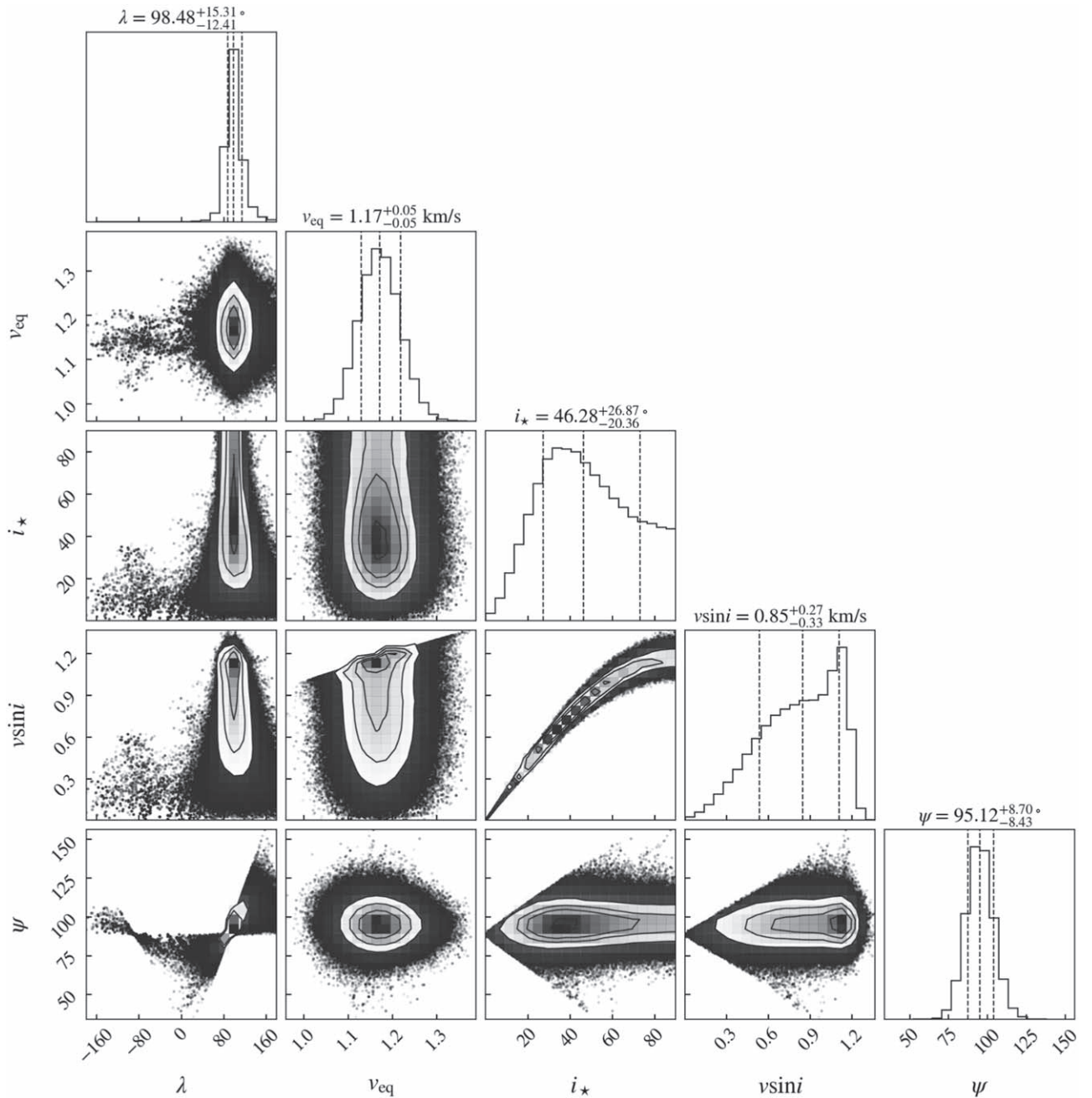
Figure 4. Corner plot of the posteriors of \lambda , v_{\text{eq}} , i_* , v \sin i , and \psi . The posteriors for the true obliquity are \psi = 95^{+9}_{-8}^\circ , and are compatible with 90^\circ for any posterior value of v \sin i .
