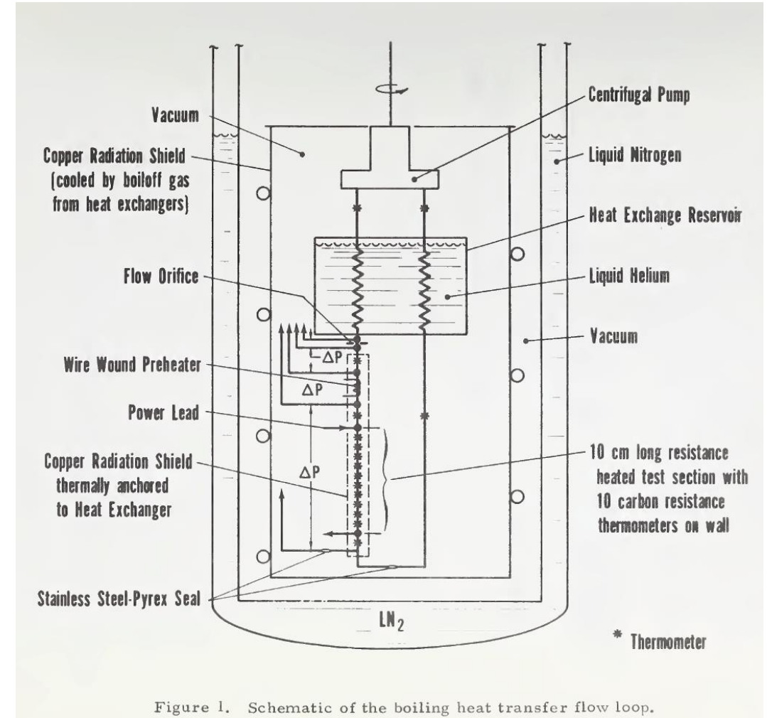
Experimental Set Up from Giarrantano et al., 1973
