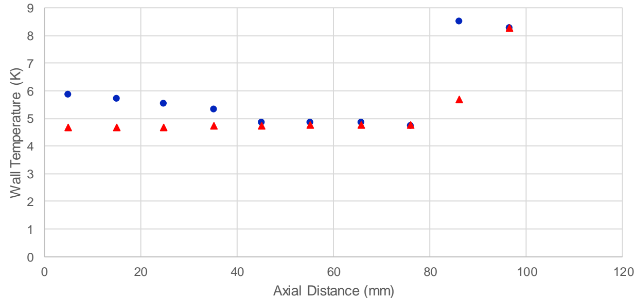
Giarrantano 1973, LHE, Run Fig 8 Sh 2 Wall Temperature
