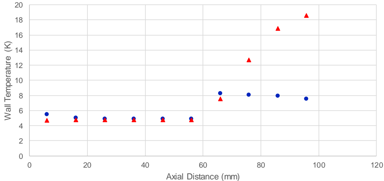
Giarrantano 1973, LHE, Run Fig 9 Sh 1 Wall Temperature
