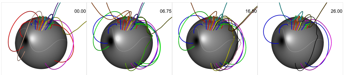
Fig. 9. Global evolution of the field lines connectivity in a pseudo-streamer topology. The color code is the same as in Figure 9: it associates a color to a particular connectivity evolution. It is the same code as in Figures 10 to 12. It is described in Sect. 3.4 to 3.6. The field lines presented here are characteristic of the nearby regions. An animation of this figure is available online.
