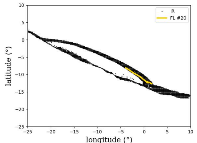
Fig. 7. Longitudinal-latitude connectivity map at 5 R_\odot displaying locations impacted by reconnection at the pseudo-streamer. The magnetic field lines connected to the black point in the figures have experienced at least one episode of magnetic reconnection during the course of the simulation. The yellow line traces the path of the intersection with the 5 R_\odot sphere of the magnetic field line n^{\circ}20 while it slip-reconnects (see Sect. 3.7).
