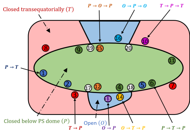
Fig. 8. Cartoon of the connectivity map at t = 0 summarizing the connectivity evolution of particular magnetic field lines during the forcing stage. The colors of the map behind the points represent all three connectivity domains at t = 0 : green for magnetic field closed below the PS dome (P), blue for open field (O), red for trans-equatorial closed field (T). The size of the equatorial coronal hole is voluntarily magnified, for readability reasons. The fixed footpoints of the selected field lines are represented by circles whose color are the same as used in Figure 9 and Figures 10 to 12. The colors correspond to particular connectivity evolution detailed in Sect. 3.4 to 3.6, depending on the connectivity states that a given field line has among P, T, and O states. For example T \rightarrow P means the field line was a trans-equatorial loop before the reconnection and a pseudo-streamer loop after the reconnection.
