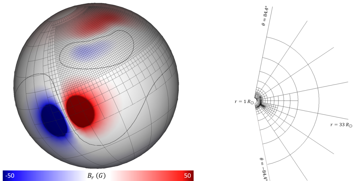
Fig. 1. Left: radial magnetic field distribution on the solar surface with a strong dipole at the equator and four weaker dipoles at higher latitudes in the northern hemisphere. The two thick black lines represent the equatorial and parasitic dipole polarity inversion lines. Right: Longitudinal 2D Sections of the grid at \Phi = -175^\circ and 5^\circ after the relaxation (see 2.4). On both panels, the simulation grid is represented with thin lines black.
