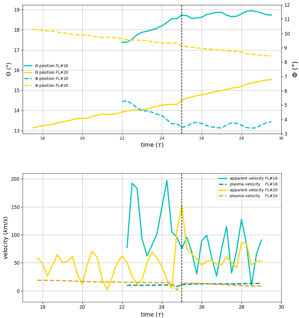
Fig. 14. Top: evolution of the \Theta (latitude, solid line) and \Phi (longitude, dashed line) components of the field lines n°16 (cyan) and 20 (yellow) at 2 R_{\odot} . Bottom: tangential velocity of the field lines n°16 (cyan) and 20 (yellow) calculated at 2 R_{\odot} between t = 17.75 \tau and t = 29.25 \tau . The cyan and yellow dashed lines display the tangential plasma velocities at 2 R_{\odot} at the location of the footpoints of the associated field lines. The vertical dashed back line indicates the end of the large, rather straight slipping motion for the cyan field line (n°16) and the beginning of the oscillations.
