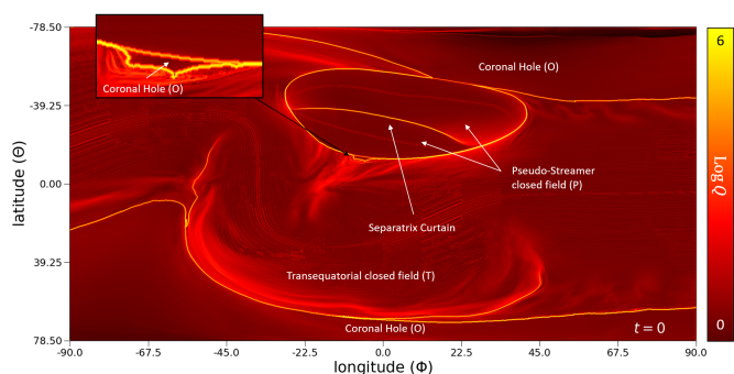
Fig. 3. Distribution of \log Q after the relaxation. The yellow-colored separatrices delineate the connectivity domains: transequatorial streamer loops, pseudo-streamer loops (both closed field), polar and equatorial coronal holes (open field). The size of the equatorial coronal hole (see inserted panel) is significantly reduced during the relaxation.
