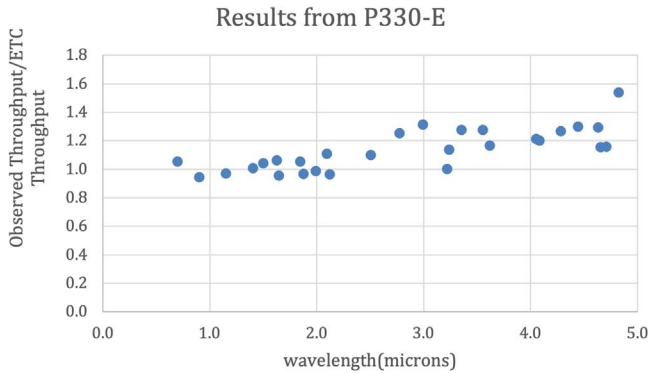
Figure 9. NIRCam imaging throughput compared to what was assumed in the pre-launch ETC. For most filters, the observed throughput is higher than the pre-launch expectations. Data are from spectrophotometric standard star P330-E observed in program PID 1074.
