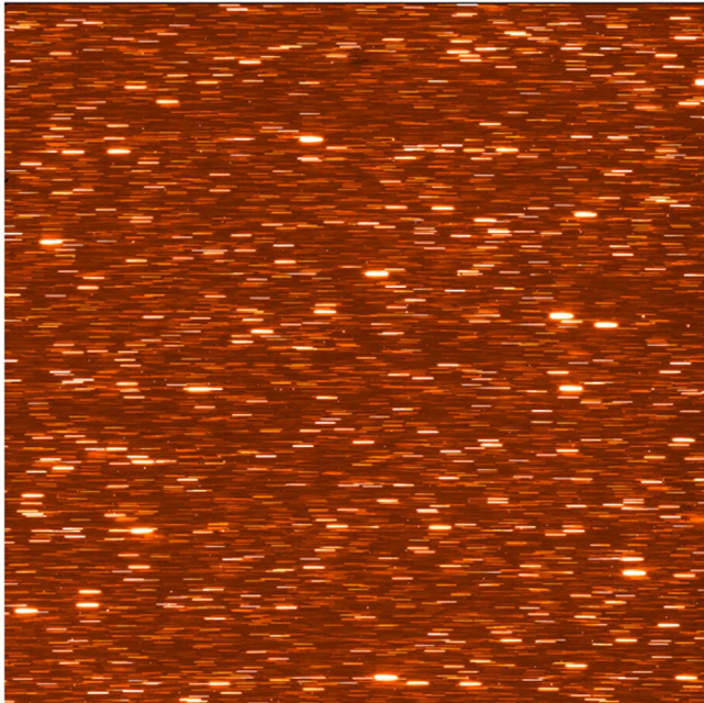
Figure 13. NIRISS WFSS. Simultaneous spectroscopy of thousands of stars in the NIRISS focus field of the LMC. Configuration is grism GR150C and filter F115W. The field of view of the detector is 2\frac{1}{2} on a side. Data from PID 1085.
