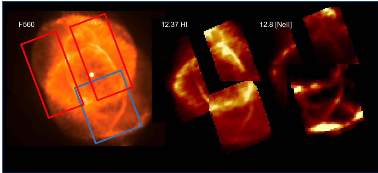
Figure 16. NGC 6543, the Catseye planetary nebula, imaged at 5.6\ \mu\text{m} (left panel), and dissected by the MIRI MRS in mosaics using its integral field unit (right two panels). The maximum extent of the nebula in the image is \sim 25'' . The two layers in the spectral/spatial cube show the nebula at sub-arcsecond resolution in Humphreys \alpha 12.37\ \mu\text{m} and the fine structure line of [\text{Ne II}] 12.8\ \mu\text{m} . MRS has four integral field units; the field of view increases with wavelength. Data are from programs PID 1023, 1031, and 1047. Credit: B. Vandenbussche
