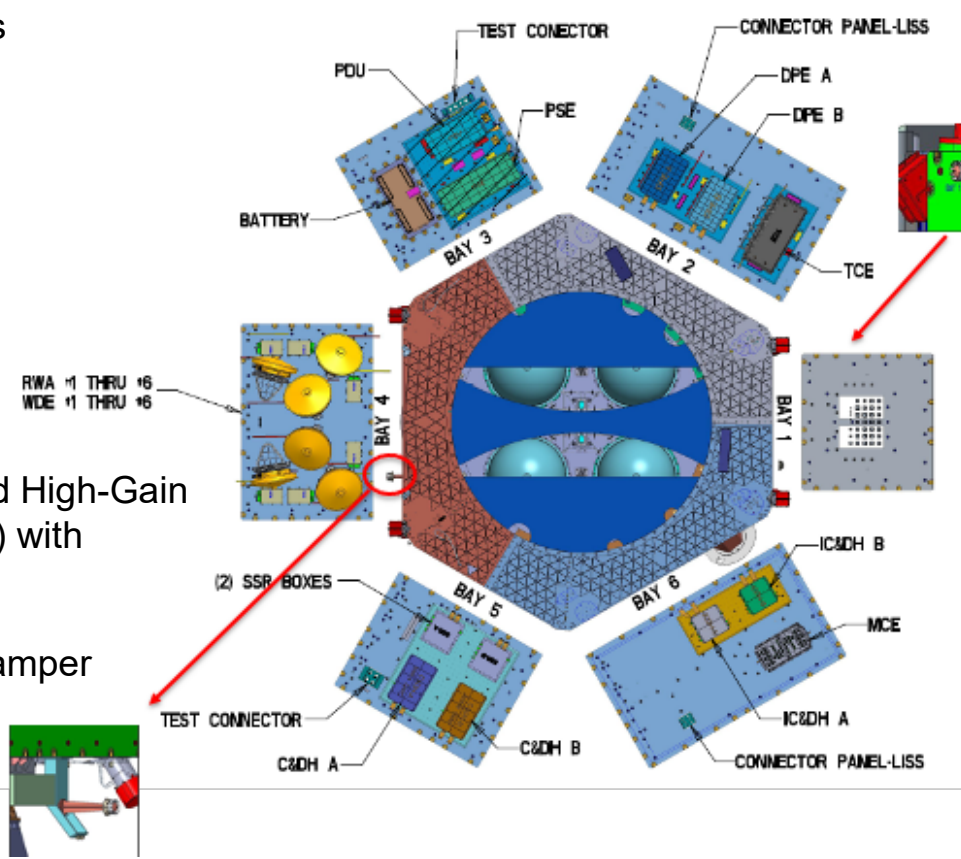
Spacecraft Bus
