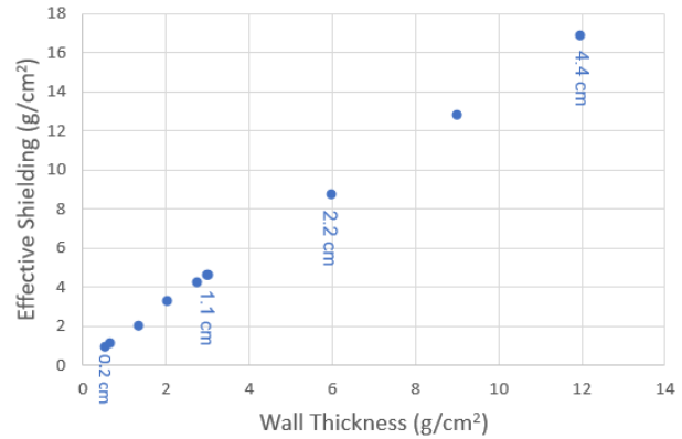
Figure 3. Generic 3U CubeSat with four electronic boards effective shielding as a function of wall thickness, showing a linear relationship.
