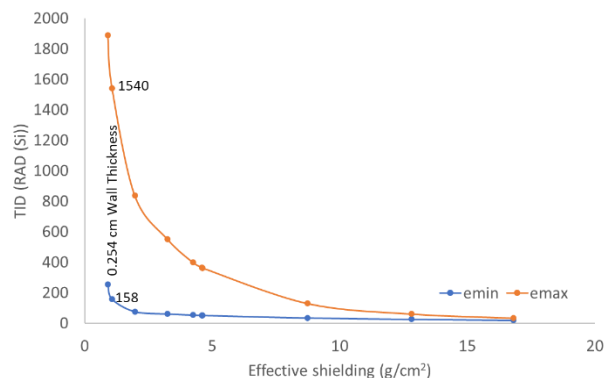
Figure 4. Generic 3U CubeSat Thin-Walled Aluminum Structure with a 10-times increase in TID from solar minimum (emin) to maximum (emax).
