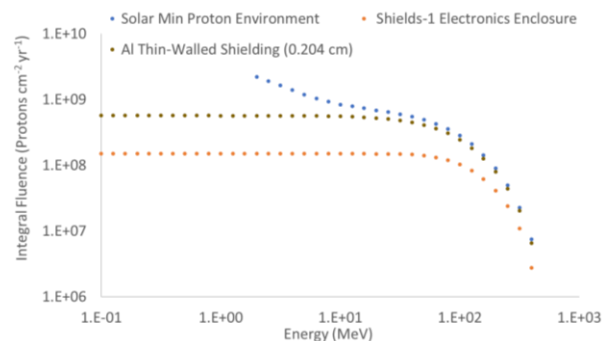
Figure 6. Proton fluences of the AP8 solar minimum environment, the Shields-1 electronics enclosure (vault), and the Al thin-walled shielding (0.204 cm). The total number of protons/cm 2 in the AP8 minimum or shielded environment for each plot is the highest Y-axis value.
