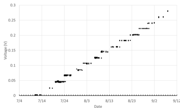
Figure 5. The Shields-1 electronics enclosure (vault) Teledyne \mu Dosimeter high-count channel, where the step increases correspond to 0.94 +/- 0.04 RAD/step. The dose occurred over a 2-month period. 10
