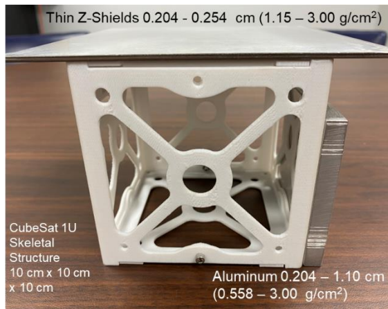
Figure 2. A comparison of thin Z-Shields and aluminum thicknesses for adding structural shielding mass to a CubeSat 1 unit (U). Thin Z-Shields enables increased mass thickness. (Image Credit: NASA)
