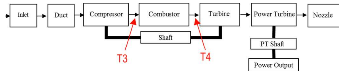
Figure 1. Simple, single-shaft turboshift with free power turbine.
