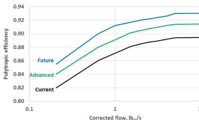
Figure 2. Turbomachinery polytropic efficiency characteristics.
