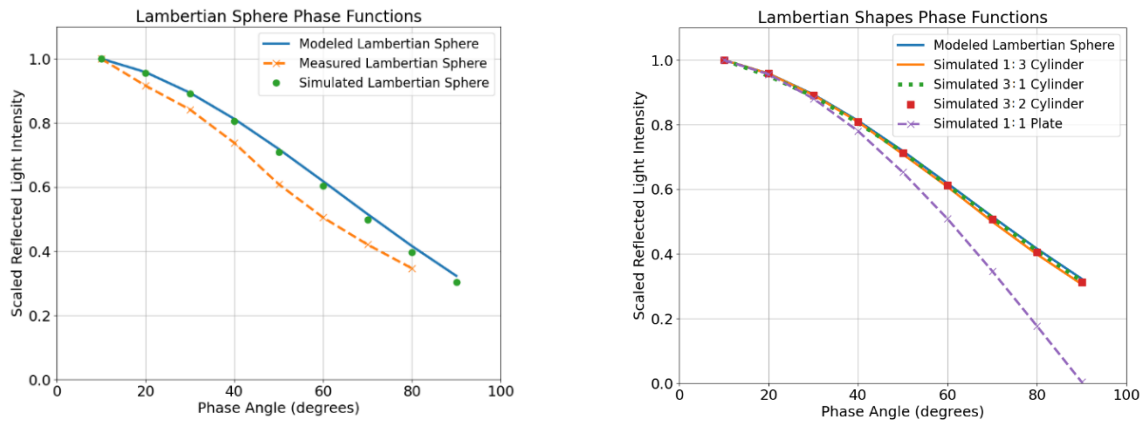
a) b) Fig. 10. a) Phase angle plot of modeled, measured, and ray-trace simulated Lambertian spheres with their scaled light intensities b) Phase angle plot of a modeled Lambertian sphere compared to ray-trace generated simulated Lambertian shapes with various L:D ratios, specifically cylinders and a plate
