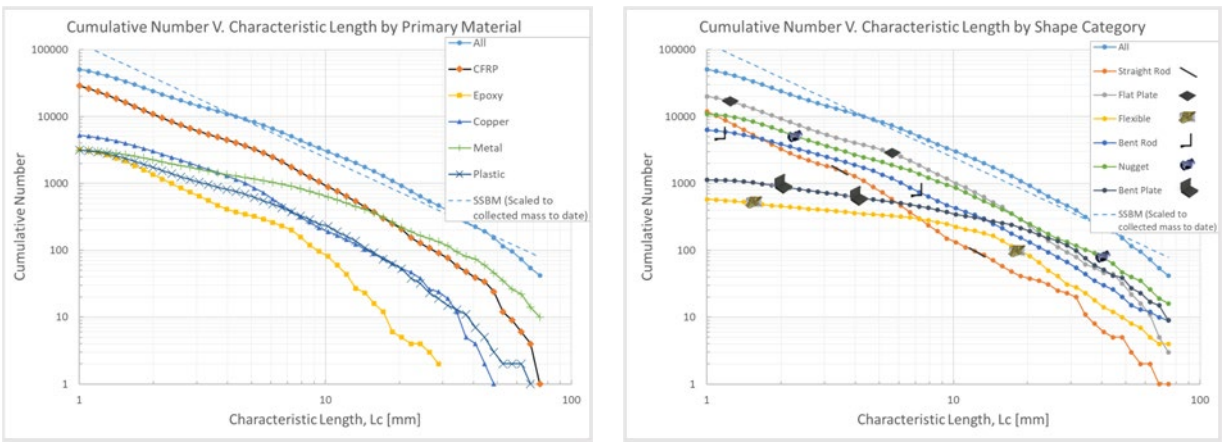
a) b) Fig. 2. Shape distributions as a function of size, as of 01 January 2023, a) is DebrisSat distribution as function of primary materials and b) is a distribution as function of shape
