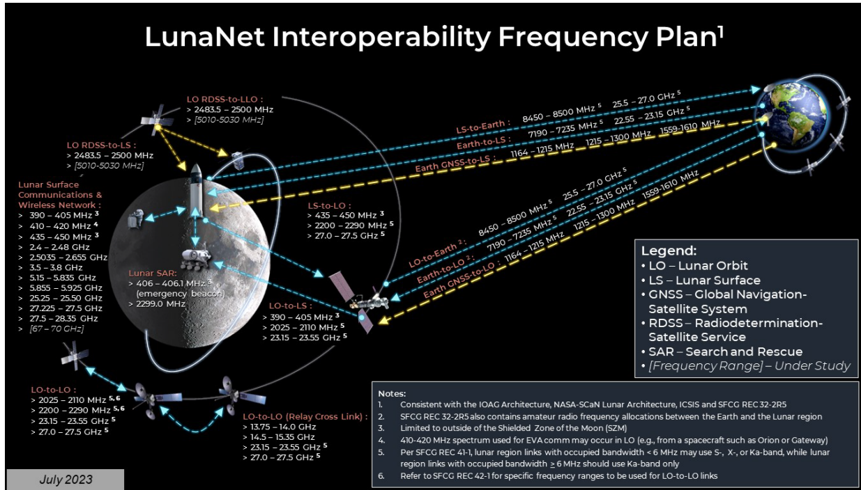
Figure 18: LunaNet Interoperability Frequency Plan
