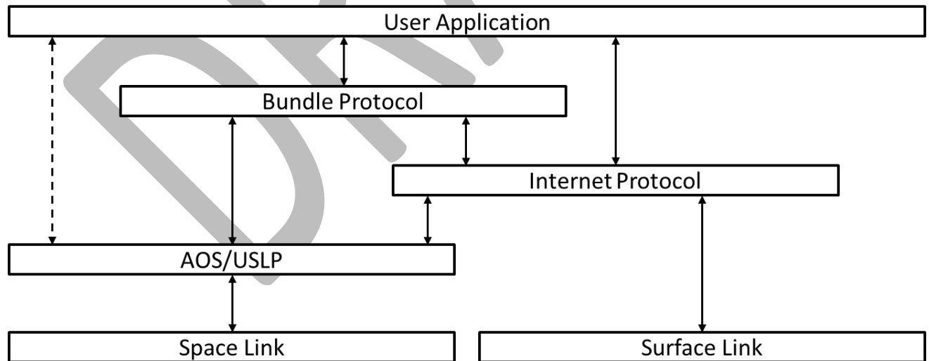
Figure 5: User Application Simplified Protocol Stack
