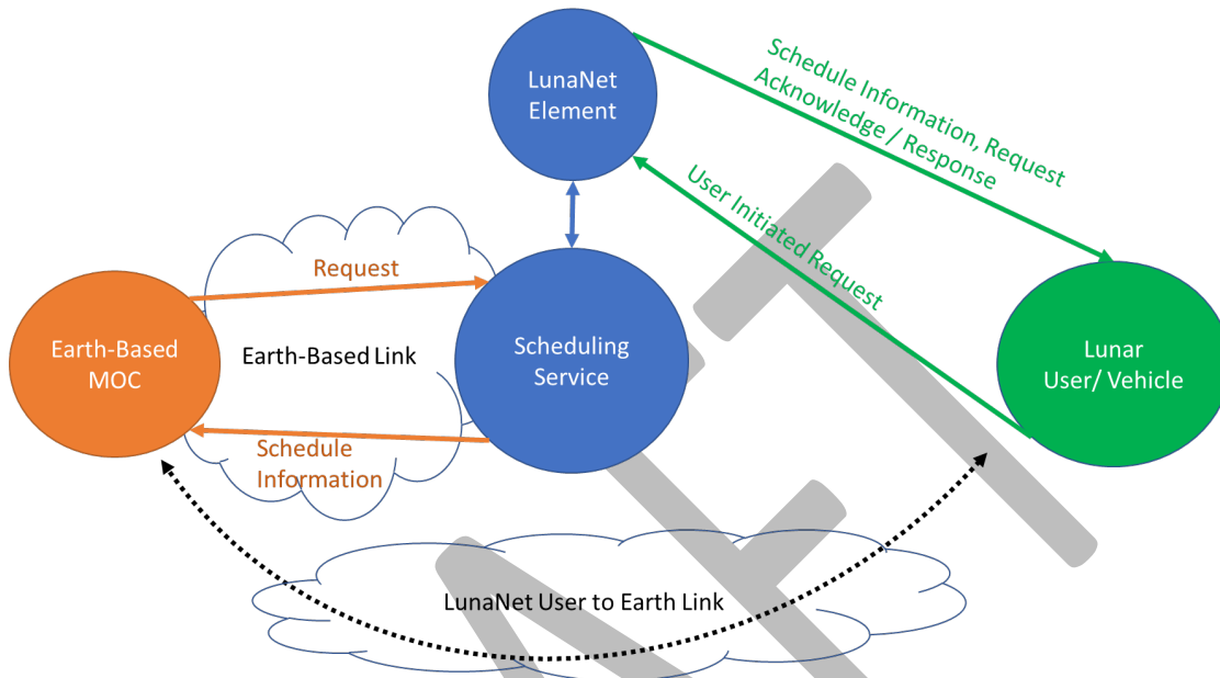
Figure 16: LunaNet Scheduling Interfaces Overview
