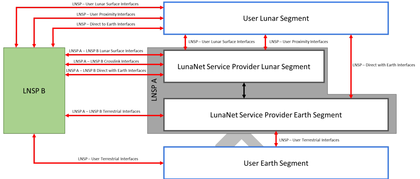
Figure 3: LunaNet Service Providers Interfaces
