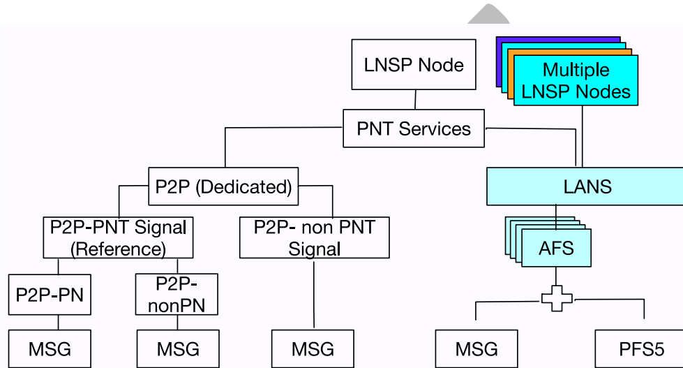
Figure 6: PNT Services Provided by LNSP
