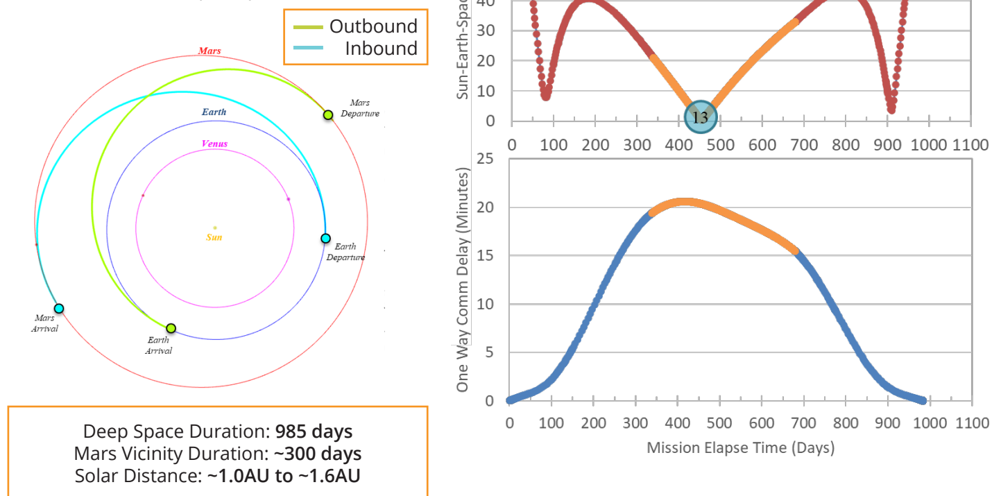
Figure 3. Communications disruption and delay profile of a representative minimum energy, approximately 1,000-day stay, roundtrip mission to Mars with a communications blackout of about 13 days and a maximum one-way communications delay of 21 minutes. Both occur while the crew is in Mars orbit or on the surface of Mars.
