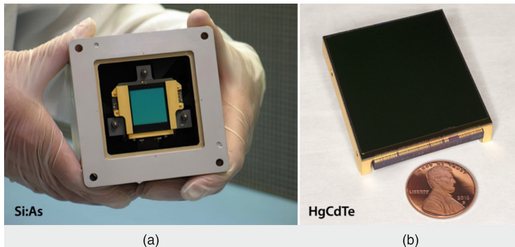
Fig. 1 State of the art mid-infrared detectors: (a) Si:As detector array used in the JWST/MIRI instrument and (b) HgCdTe long-wavelength detector ( \lambda > 10 \mu\text{m} ) to be used in the NEOSM.
