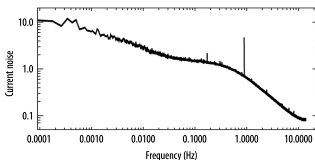
Fig. 3 Long duration laboratory measurement of the average noise spectrum of a GSFC TES detector array (in units of normalized current noise density).
