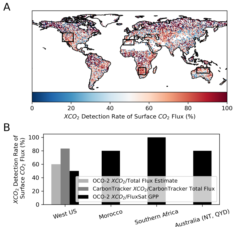
555 Figure 8. OCO-2 XCO 2 anomalies alone can detect extreme CO 2 flux anomalies. OCO-2 detection rate of extreme surface CO 2 flux anomalies (or positive XCO 2 anomalies when surface CO 2 efflux anomalies are the largest) (a) across the globe in each pixel and (b) within specific regions. The legend in (b) shows the datasets used to estimate the detection rate including pairs of OCO-2 XCO 2 anomalies and total CO 2 flux anomaly estimates from LPJ and QFED, pairs of CarbonTracker XCO 2 anomalies and CarbonTracker total CO 2 flux anomaly estimates, and pairs of OCO-2 XCO 2 anomalies and photosynthesis flux anomaly estimates from FluxSat GPP.
