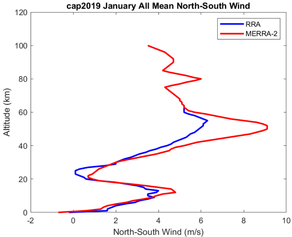
Figure 6. Plot of January mean north-south comparison between MERRA-2 and Cape Canaveral, FL RRA.
