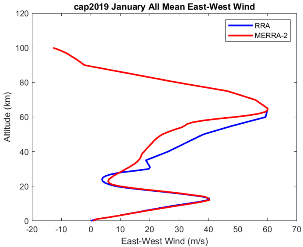
Figure 5. Plot of January mean east-west wind comparison between MERRA-2 and Cape Canaveral, FL RRA.
