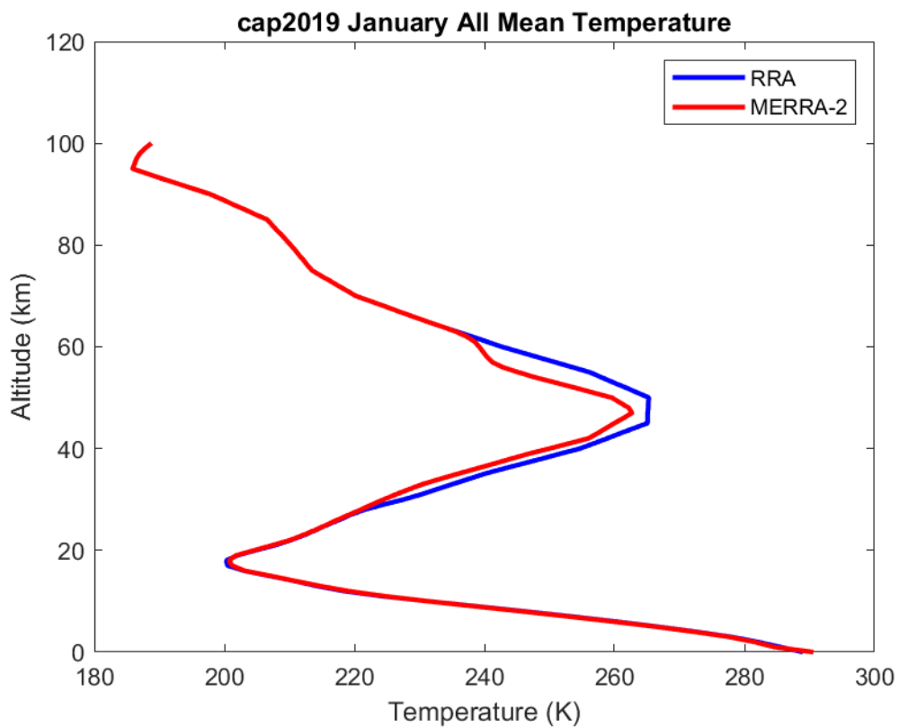
Figure 3. Plot of January mean temperature comparison between MERRA-2 and Cape Canaveral, FL RRA.
