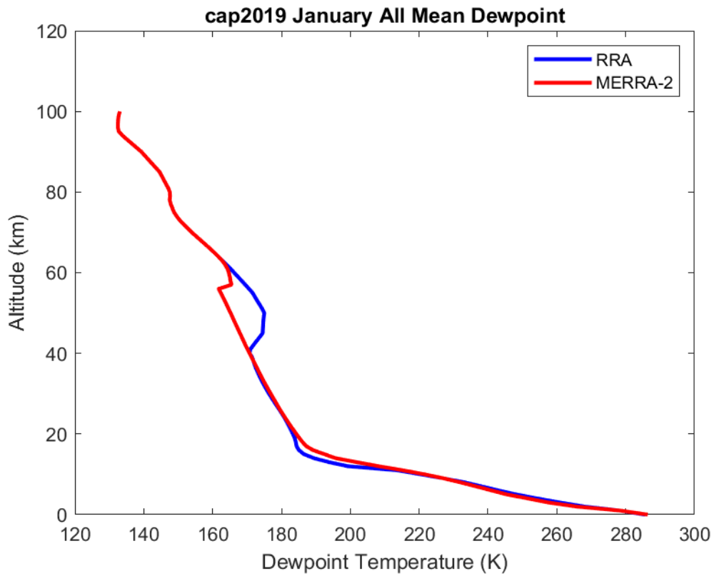
Figure 4. Plot of January mean dewpoint comparison between MERRA-2 and Cape Canaveral, FL RRA.
