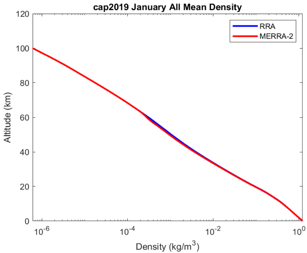
Figure 2. Plot of January mean density comparison between MERRA-2 and Cape Canaveral, FL RRA.
