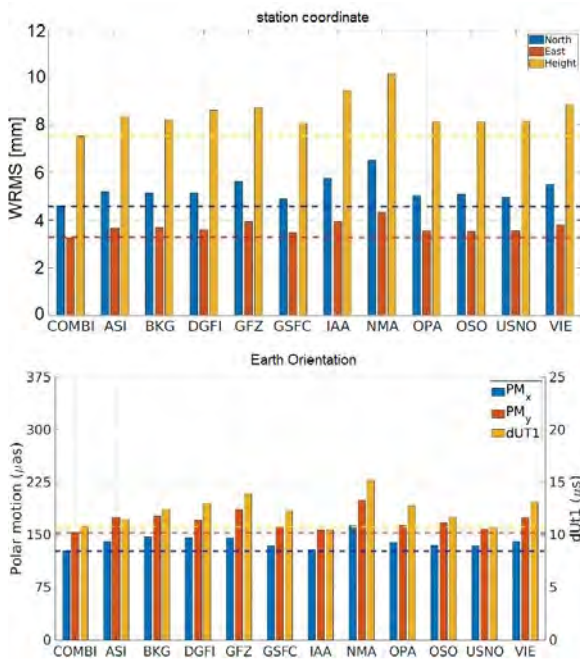
Fig. 1 Station coordinate WRMS of all stations (upper figure). WRMS for Polar Motion and dUT1 (lower figure).
