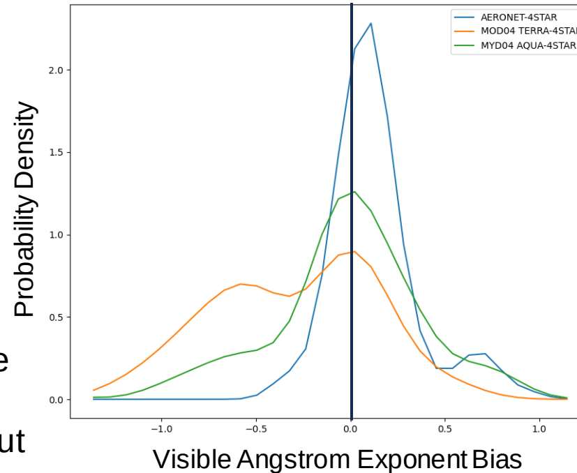
Standard MODIS Retrievals
