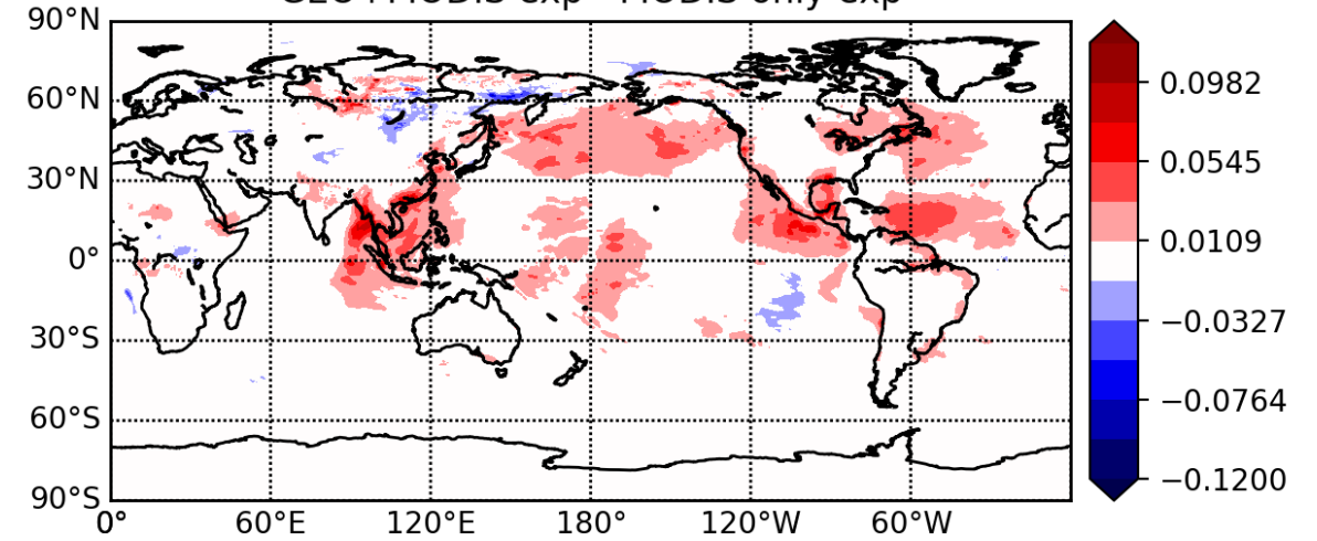
GEO+MODIS exp - MODIS only exp
