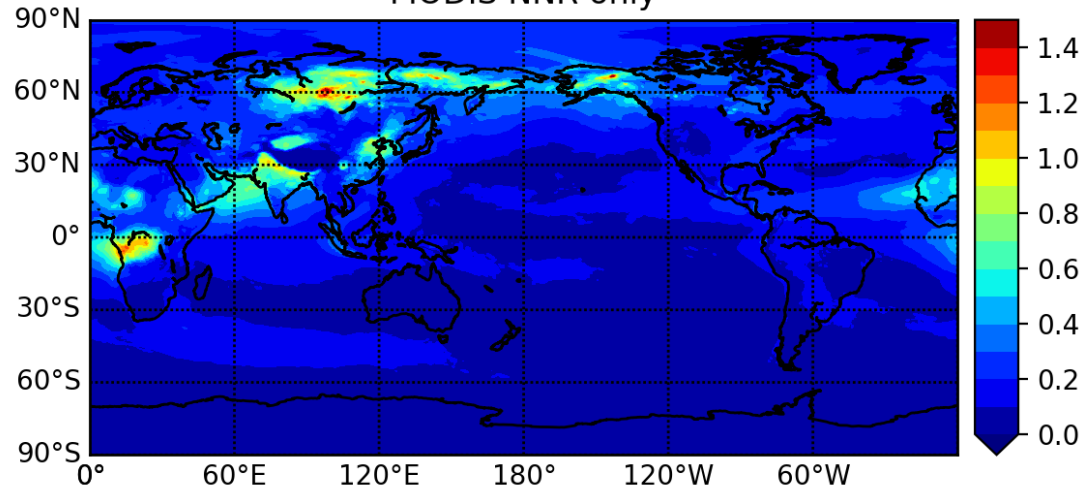
MODIS NNR only
