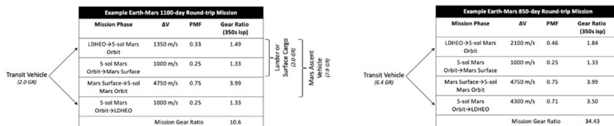
Figure 4. Gear Ratios for 850-Day and 1,100-Day Crewed Round-Trip Mars Missions
