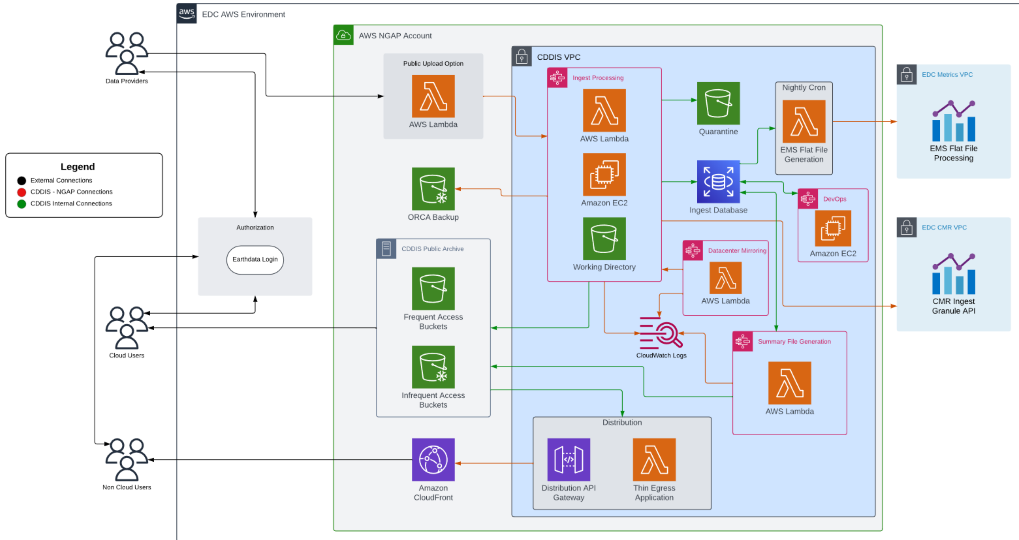
Figure 3: The CDDIS Flow Diagram for onboarding to the Cloud
