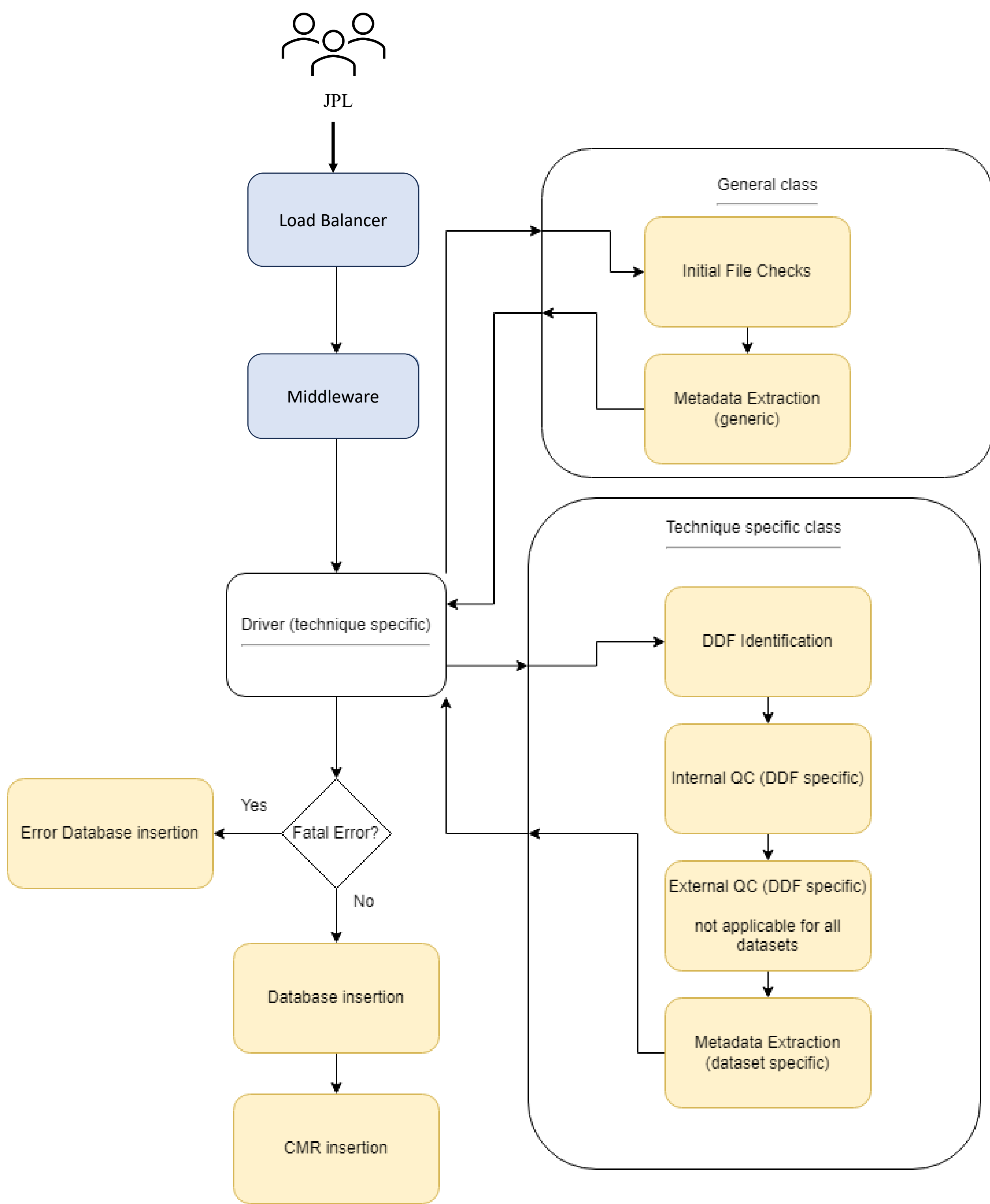
Figure 1: The CDDIS Processing V4 Software Flow Diagram
