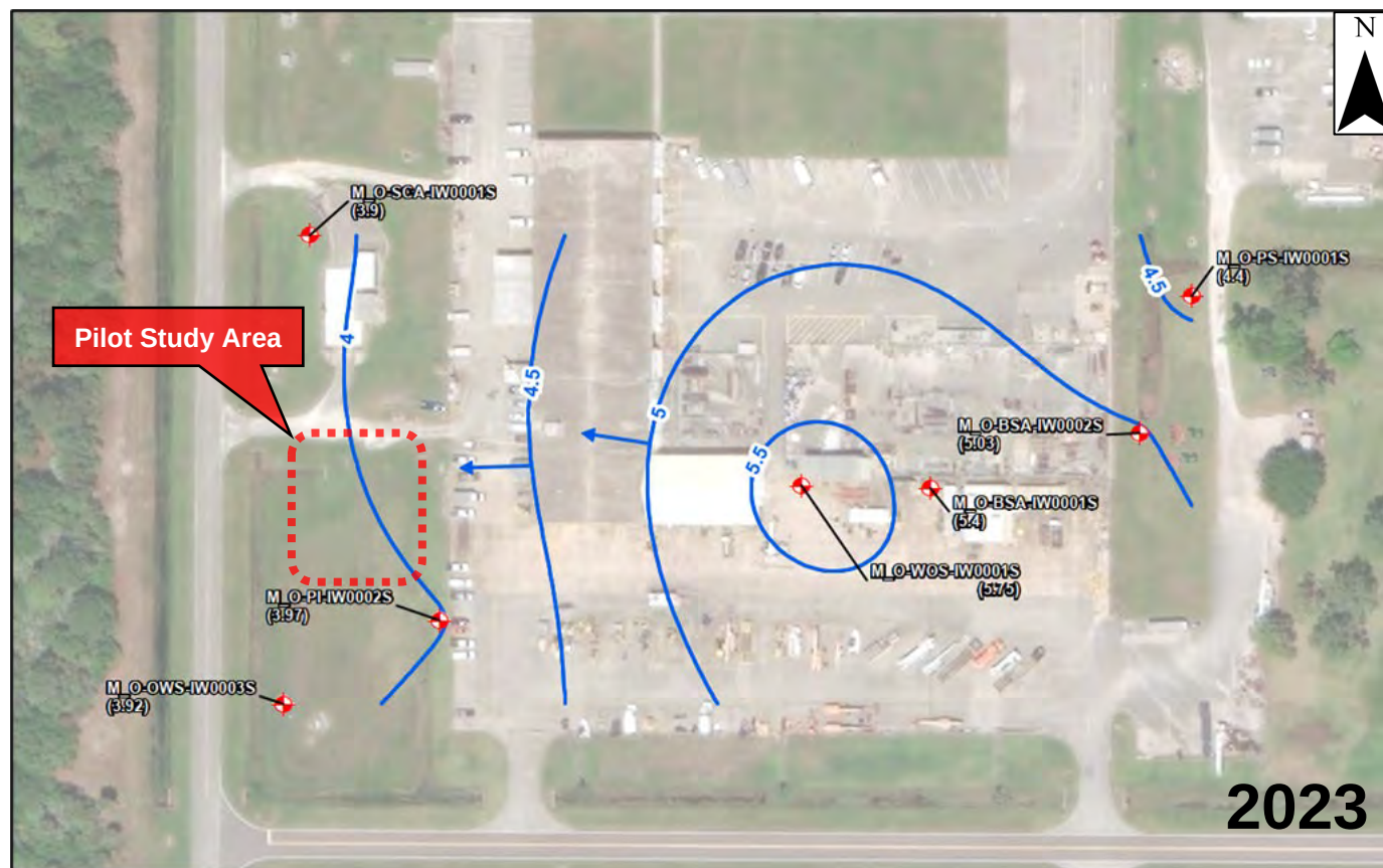
Groundwater elevation data collected by HydroGeoLogic in April 2023. Figure created by AECOM in August 2023.
