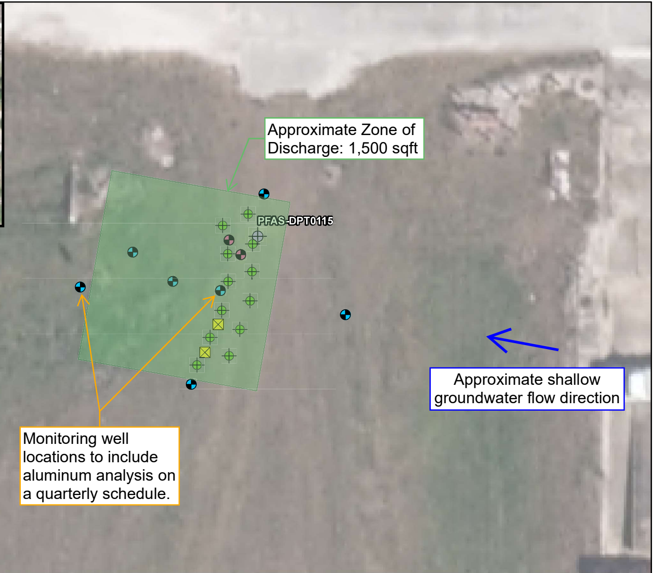
FIGURE 2-1 Base Support Building PlumeStop® Injection Pilot Study Layout JOHN F. KENNEDY SPACE CENTER MERRITT ISLAND, FLORIDA
