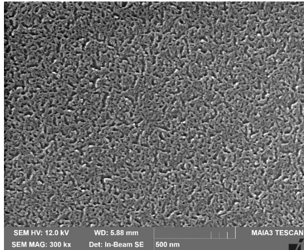
Figure 46. FESEM images the Kapton H layer of the M12Z-Z1 F AO Photo Monitor. (a) 200X at the exposed-protected border, (b) 300kX in the protected region, and (c) 300kX in the exposed region.
