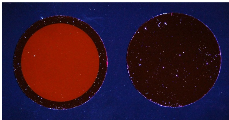
Figure 34. Post-flight photographs of M10R-C1 F and M10R-C1 B. (a) Visible light image with both Part A (top layer) and Part B (bottom layer), (b) Visible light image (M10R-C1 F Part A on left and M10R-C1 B Part A on the right), and (c) UV light (365 nm) image with M10R-C1 F Part A on left and M10R-C1 B Part A on the right.
