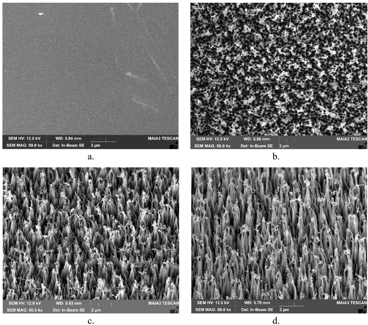
Figure 44. FESEM images the Kapton H layer of the M12R-R2 F AO Photo Monitor. (a) Protected region at 0° tilt (80kX), (b) Exposed region at 0° tilt (80kX), (c) Exposed region at 30° tilt (80kX), and (d) Exposed region at 45° tilt (80kX).
