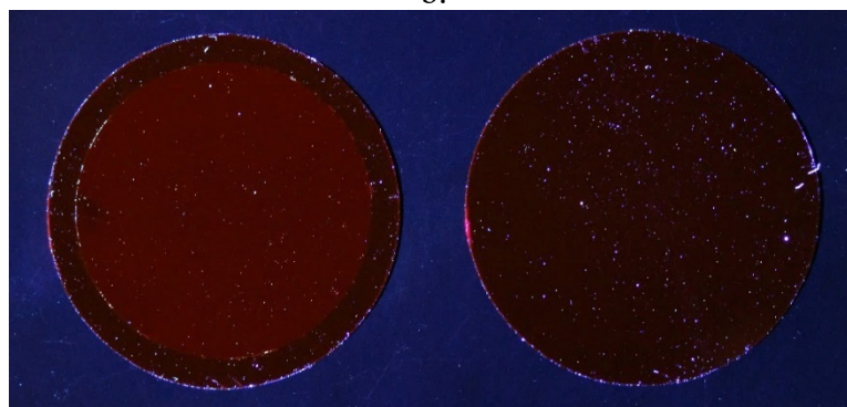
Figure 35. Post-flight photographs of M10Z-C1 F and M10Z-C1 B. (a) Samples on a white background, (b) Visible light image of samples on a dark background (M10Z-C1 F on the left and M10Z-C1 B on the right), and (c) UV light (365 nm) image with M10Z-C1 F on the left and M10Z-C1 B on the right.
