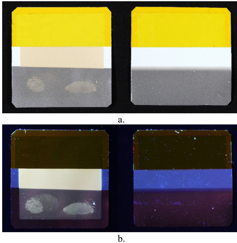
Figure 49. Post-flight photographs of M13W-S1 F (left) and M13W-S1 B (right). (a) Visible light image, and (b) UV light (365 nm) image.
