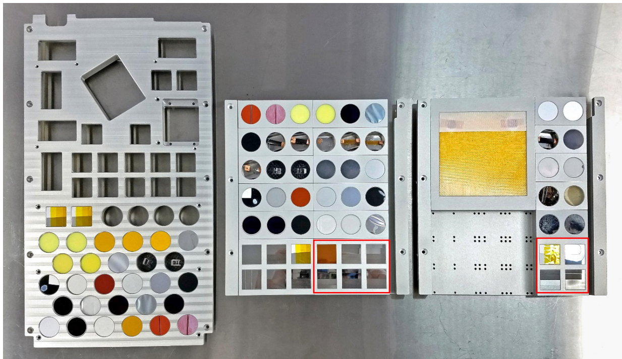
Figure 12. Pre-flight photograph of the MISSE-12 PCE-3 samples loaded into the MSC flight decks, from left to right: R2 MSC 4 SS (ram), W3 MSC 6 MS (wake), and Z1 MSC 18 MS (zenith). Samples in red boxes were moved to a different location on the deck prior to flight.
