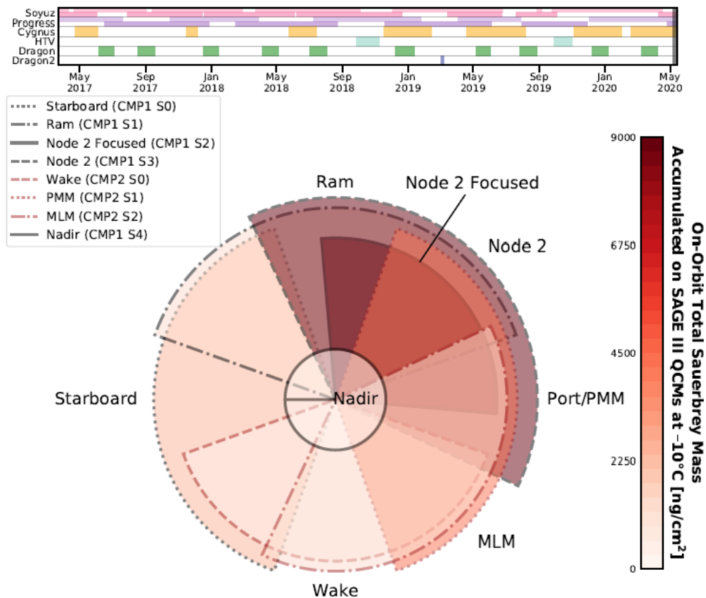
Figure 56. Contamination Deposition Map of the SAGE III Sensors from Reference 46.
