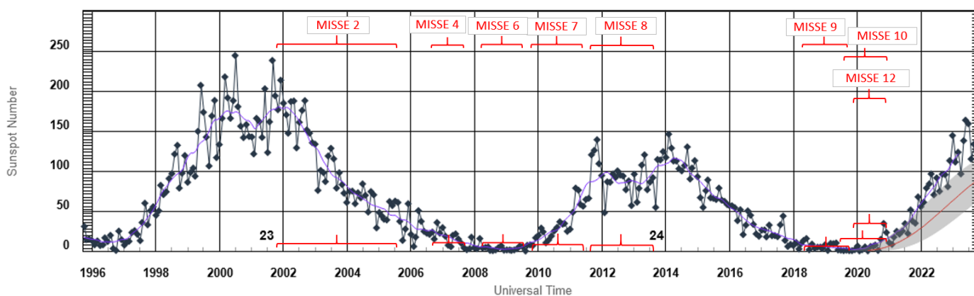
Figure 54. International Space Environmental Services (ISES) Solar Cycle Sunspot Number Progression. 45
