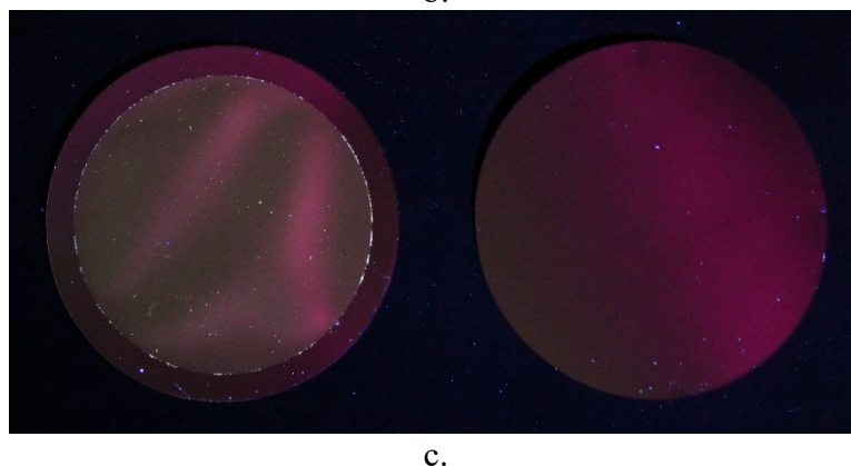
Figure 38. Post-flight photographs of M10Z-C2 F and M10Z-C2 B. (a) Samples on a white background, (b) Visible light image of samples on a dark background (M10Z-C2 F on the left and M10Z-C2 B on the right), and (c) UV light (365 nm) image with M10Z-C2 F on the left and M10Z-C2 B on the right.
