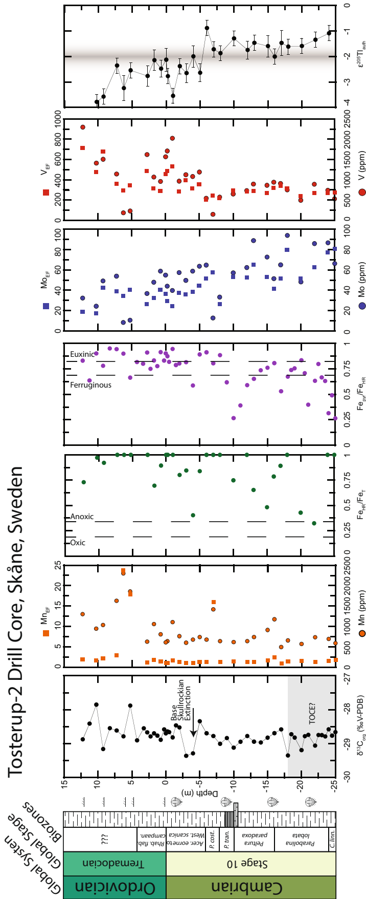
FIGURE 3 Upper Furongian and Tremadocian geochemical profiles of the Tosterup-2 drill core. Trilobite (Cambrian) and graptolite (Ordovician) biozones are plotted from previous biostratigraphic studies (Terfelt et al., 2014). Horizontal gray bar indicates the putative TOCE negative excursion. Vertical gray bar represents bulk crustal isotopic value of TI
