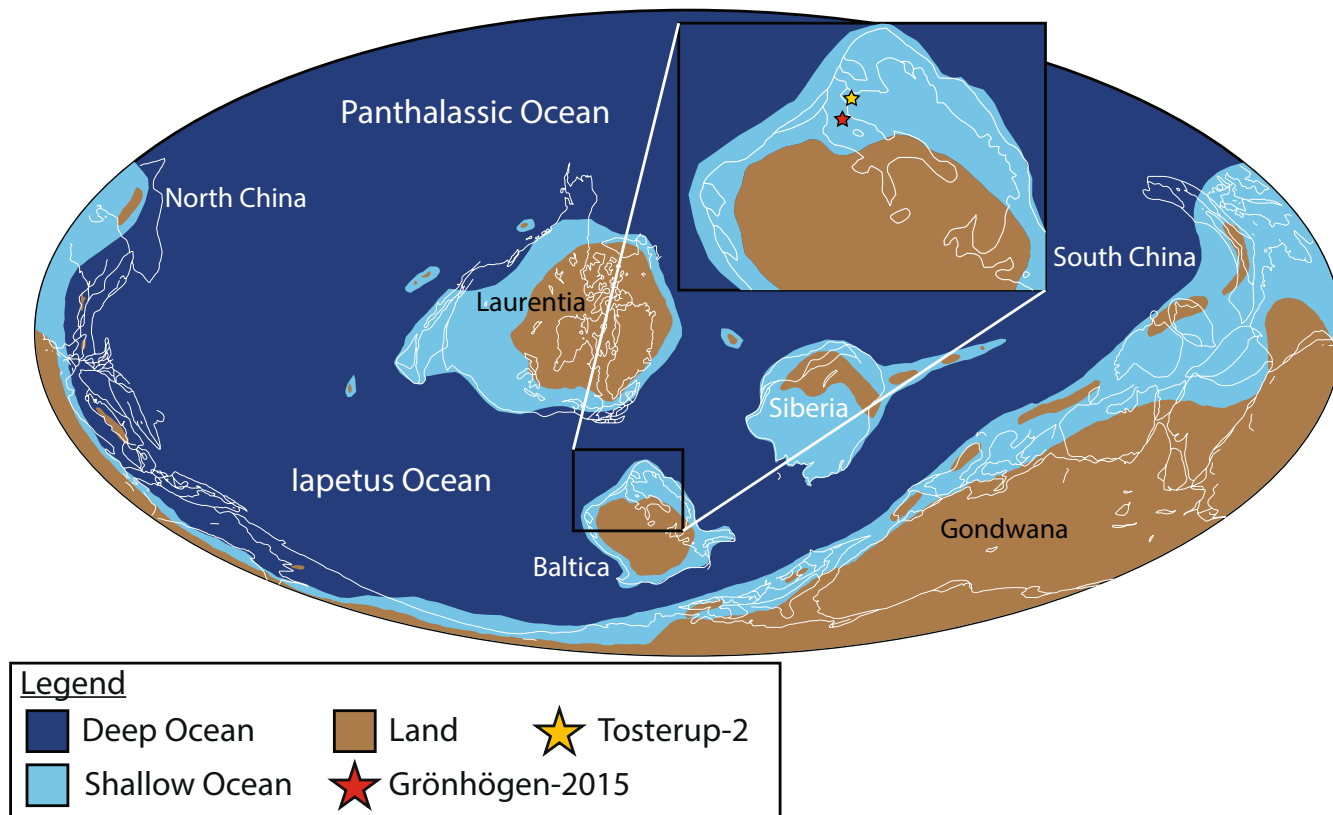
FIGURE 1 Paleogeographic reconstruction of the late Cambrian with approximate location of study sites marked in red and yellow stars. Modified from Scotese (2001). [Correction added on 02 February 2023, after first online publication: Figures 1 to 6 has been updated with the revised version]
