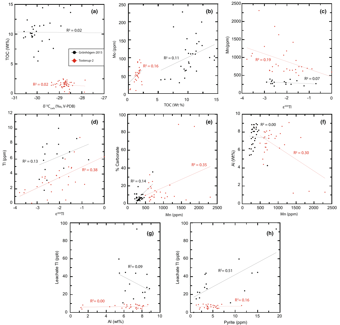
FIGURE 4 Cross-plots of geochemical data used for diagenetic alteration screening. Black circles indicate geochemical data from the Grönhögen-2015 core, and red diamonds indicate geochemical data from the Tosterup-2 core
