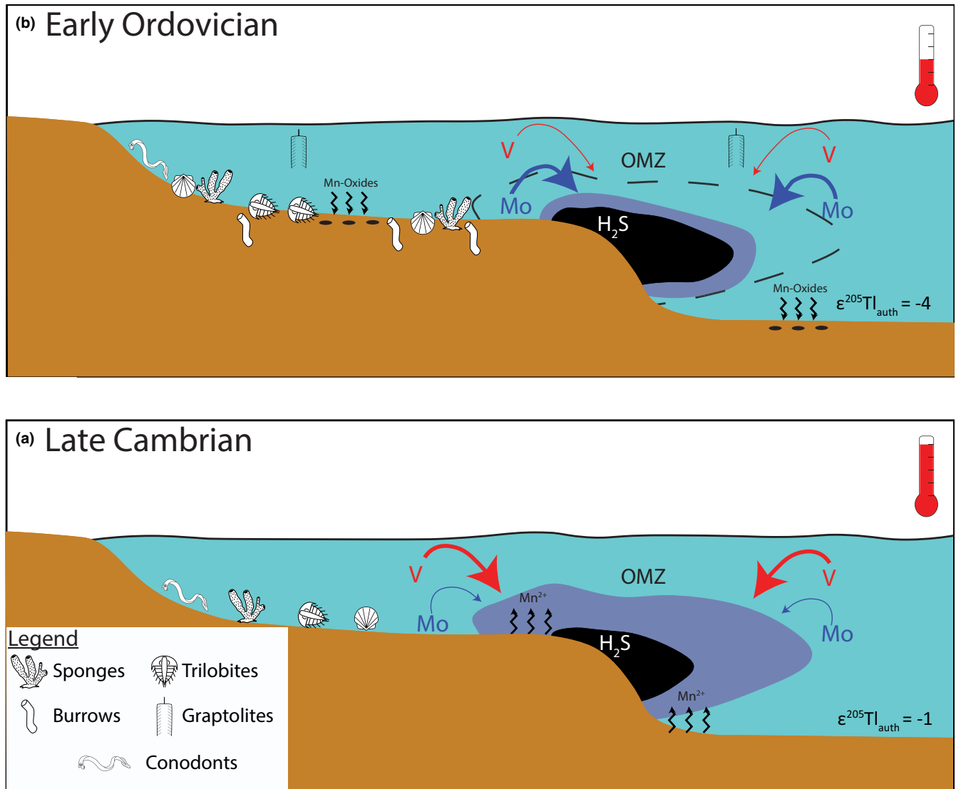
FIGURE 5 Reconstruction of typical late Cambrian and Early Ordovician margins. Changes in anoxic (purple) and euxinic (black) extent are based on V and Mo dynamics as discussed in the text. Changes in Mn-oxide formation and burial are based on TI isotopic changes. The late Cambrian is characterized by largely reducing conditions, and an overall reduced capacity for form and bury Mn-oxides when compared to the Early Ordovician. The release of aqueous Mn^{2+} would occur wherever condition do not allow for the long-term burial of Mn-oxides. The relative abundance of fauna indicates relative changes in biodiversity of that faunal group
