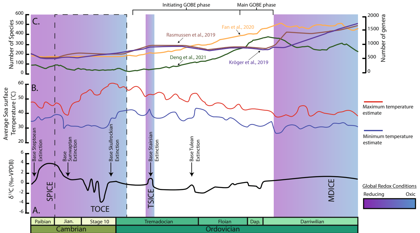
FIGURE 6 Summary of geochemical and physical palaeoceanographic trends of the late Cambrian–Early Ordovician. (a) Generalized \delta^{13}\text{C}_{\text{carb}} trends of the late Cambrian–Middle Ordovician. (b) Generalized average sea surface temperature ranges for the late Cambrian–Middle Ordovician. Upper red line represents the maximum temperature estimates while the lower blue line represents minimum temperature estimates (modified from Goldberg et al., 2021). (c) Generalized biodiversity trends of the late Cambrian–Middle Ordovician, modified from Deng et al. (2021). Species axis refers to biodiversity trends of Deng et al. (2021) and Fan et al. (2020) (green and orange lines, respectively), while genera axis refers to trends from Rasmussen et al. (2019) and Kröger et al. (2019) (brown and purple lines, respectively). Gradients from purple to blue represent changes from globally reducing conditions (purple) to more oxygenated global conditions (blue). Dashed box surrounding the late Cambrian–Early Ordovician represent our study interval
