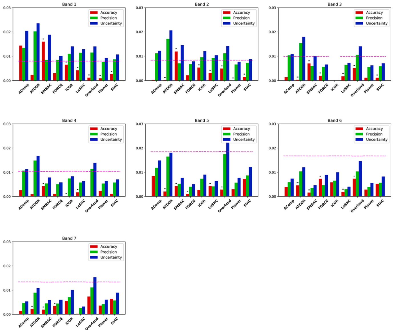
Fig. 10. Accuracy (Red), Precision (Green), Uncertainty (Blue) surface reflectance analysis results over all 110 AERONET sites. The specification ( 0.05p + 0.005 ) is displayed with the magenta dashed line and is calculated using the average reference surface reflectance for each processor and band. The minus sign (–) over the bars refers to the negative values of the metric. (For interpretation of the references to colour in this figure legend, the reader is referred to the web version of this article.)
