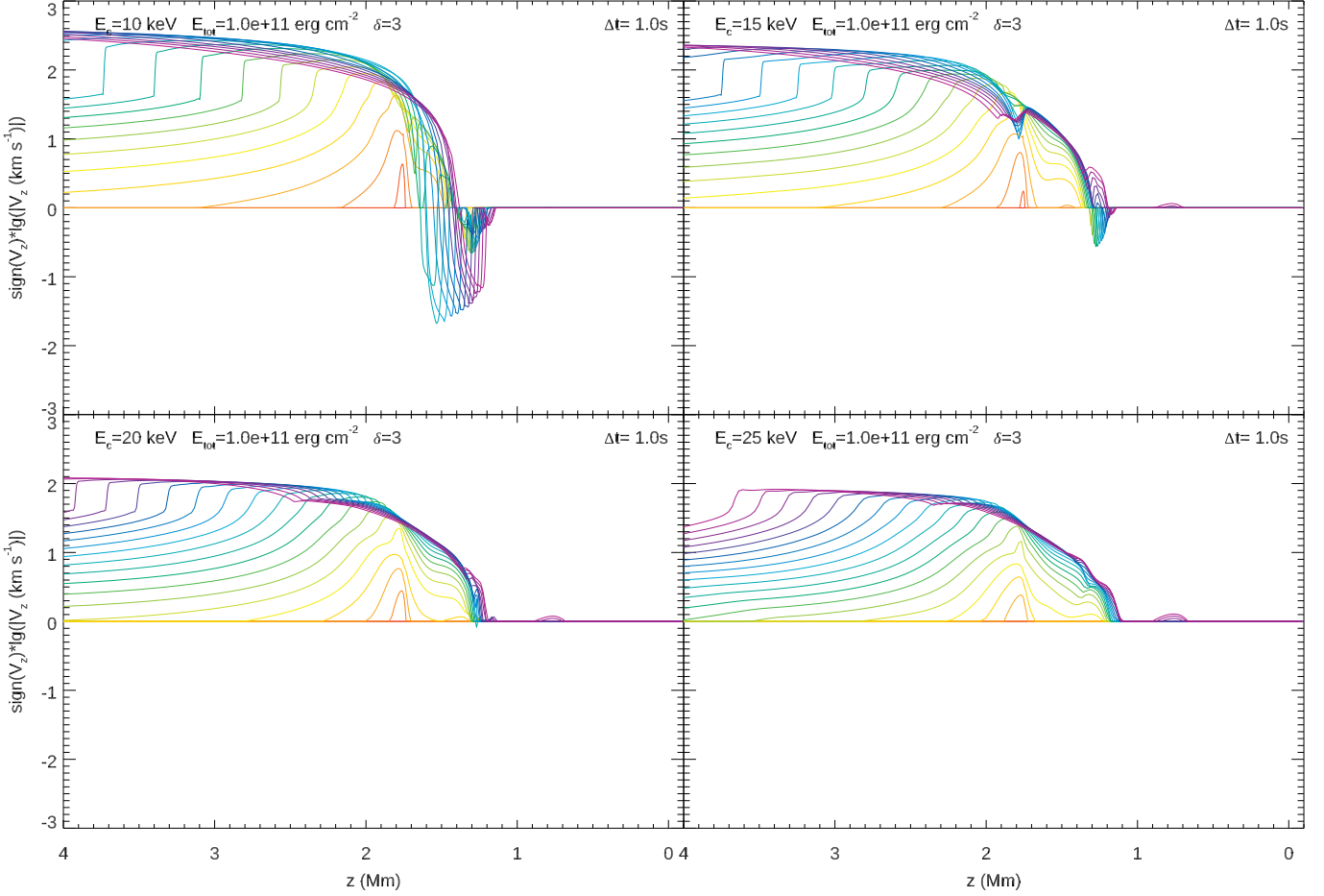
Fig. 6. Bulk velocity as function of loop position, z , and time for the four different values of the low-energy cutoff, a total energy of 10^{11} \text{ erg cm}^{-2} , and a spectral index of 3. The logarithm of the absolute value of the bulk velocity is shown, multiplied by the sign of the velocity. A value of one thus corresponds to an outflow of 10 \text{ km s}^{-1} , minus one to an inflow of 10 \text{ km s}^{-1} . Absolute values of the bulk velocity below 1 \text{ km s}^{-1} are shown as zero. The initial velocity of zero is shown in red, with subsequent timesteps, separated by 1.0\text{s} , shown with rainbow colours from red to violet. The last timestep shown is at t=20\text{s} , when the beam was switched off.
