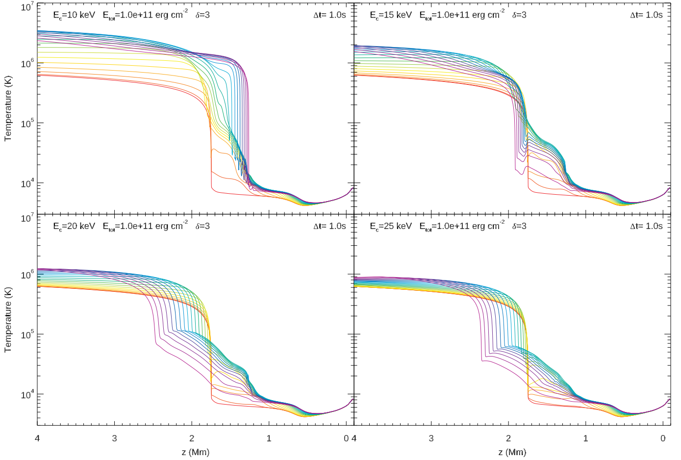
Fig. 5. Temperature as function of loop position, z , and time for the four different values of the low-energy cutoff, a total energy of 10^{11} \text{ erg cm}^{-2} , and a spectral index of 3. The initial temperature structure is shown in red, with subsequent timesteps, separated by 1.0s, shown with rainbow colours from red to violet. The last timestep shown is at t=20\text{s} , when the beam was switched off.
