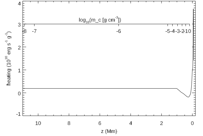
Fig. 2. Extra heating applied to sustain a VAL3C-like initial atmosphere. The constant value in the chromosphere, transition region, and corona is 1.9 \times 10^9 erg s ^{-1} g ^{-1} .
