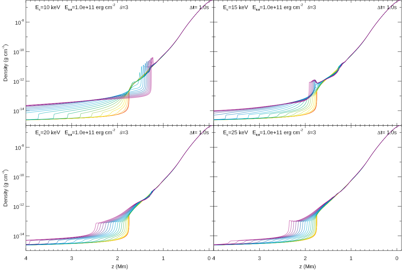
Fig. 7. Mass density as function of loop position, z , and time for the four different values of the low-energy cutoff, a total energy of 10^{11} erg cm ^{-2} , and a spectral index of 3. The initial density structure is shown in red, with subsequent timesteps, separated by 1.0s, shown with rainbow colours from red to violet. The last timestep shown is at t=20 s, when the beam was switched off.
