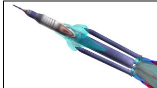
Building Aerodynamic Databases for the SLS
