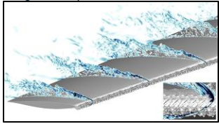
Simulating an Iced Wing for Performance Predictions
