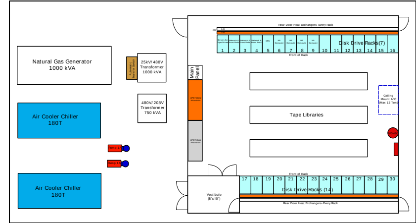
Plan View of Data Module & Infrastructure
