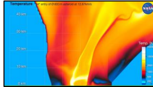
High-Fidelity Modeling of Large Asteroid Impacts
