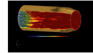
Simulating Rocket Engine Combustion of Methane-Oxygen Fuel
