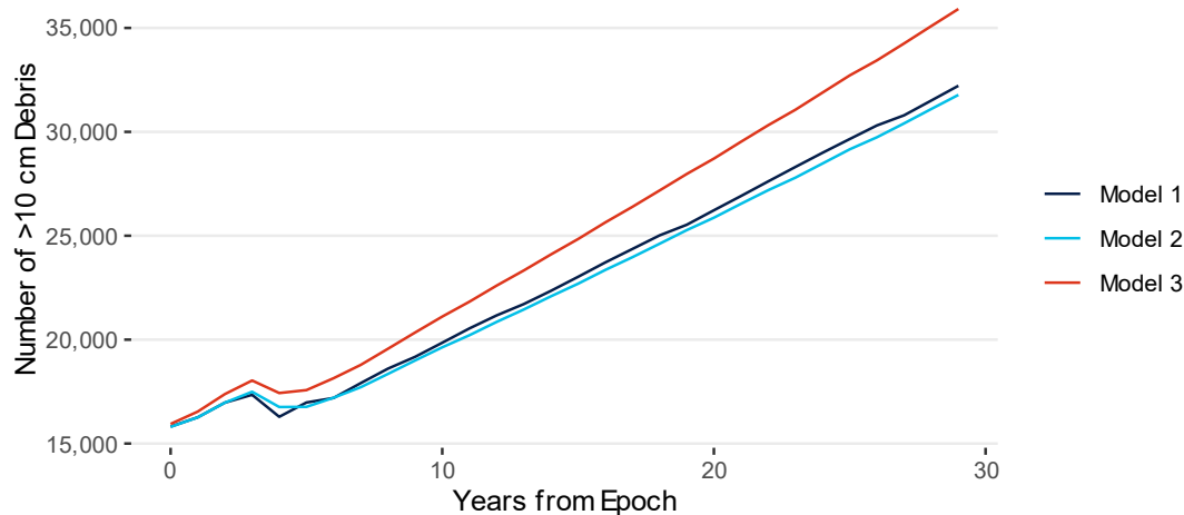
Figure A-12. Simulations of the growth of >10-centimeter debris populations. Note: The COMSPOC collision model predicts a greater representation of large debris from collisions, which explains the higher growth rate of these debris.
