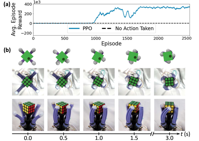
Fig. 7: (a) Reward history for the first 2,500 episodes of an In-Hand Manipulation training run with PPO. (b) Rollout of the final PPO-trained In-Hand Manipulation policy in simulation and hardware.
