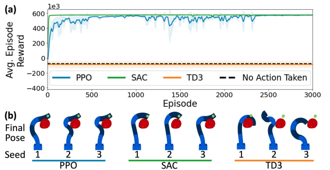
Fig. 3: Planar Reaching with Obstacle training results. (a) Reward history for the first 3000 training episodes for each algorithm. Curves are the average smoothed reward (window size 20) across three random seeds, and shaded regions indicate plus/minus one standard deviation. (b) Final pose from rollouts of the best policy developed by each seed of each algorithm. PPO and SAC learned similar policies, each reaching the (green) goal in a reliable and stable manner. Some of these policies brace against the (red) obstacle, while others reach around it. The policies trained with TD3 do not succeed in reaching the goal.
