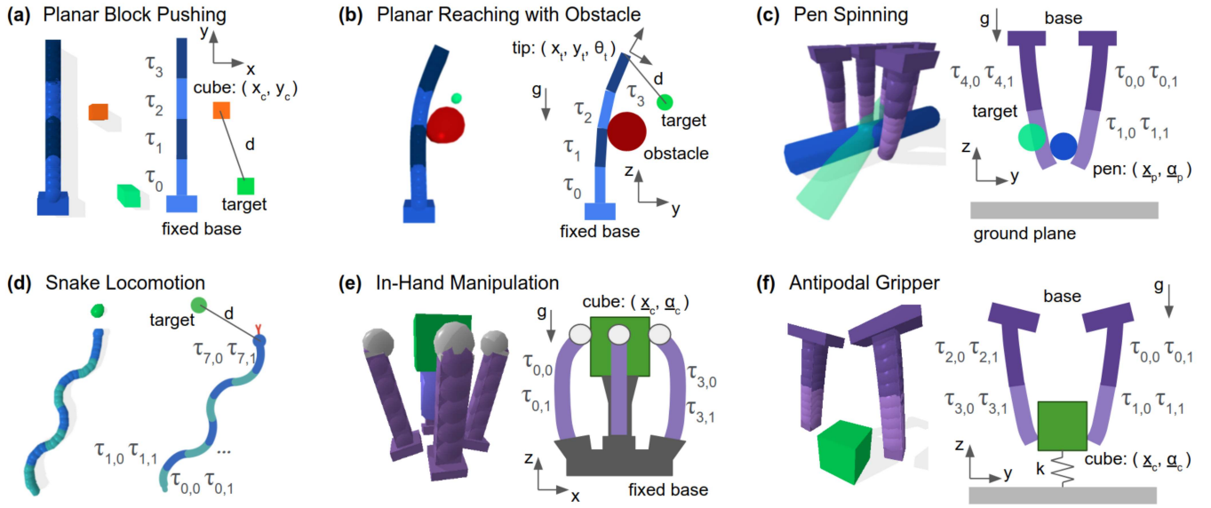
Fig. 2: SoMoGym provides a suite of benchmark tasks with soft continuum manipulators. The environments have a standardized interface similar to the one employed in OpenAI Gym, allowing for straightforward integration with common reinforcement learning frameworks. These tasks include: (a) In Planar Block Pushing , a planar continuum manipulator is tasked to move a cube to a goal position. The manipulator has four independently controlled actuators with torques \tau_i for i \in [0, 1, 2, 3] . (b) In Planar Reaching with Obstacle , the same manipulator must move its tip to a goal pose in the presence of a cylindrical obstacle. (c) In Pen Spinning , an anthropomorphic soft hand holds a cylindrical object that needs to be moved to the desired pose. The hand has five fingers, each of which has two actuators with two independently controlled torques per actuator. (d) In Snake Locomotion , a snake-like robot has to move towards a goal. The snake robot has eight independently controlled actuators with two active axes each with torques (\tau_{i,0}, \tau_{i,1}) for i \in [0, 1, 2, \dots, 7] . (e) In In-Hand Manipulation , a soft hand with four fingers is tasked to rotate a cube around the z-axis. Each of the fingers has two axes with bending torques (\tau_{i,0} and \tau_{i,1}) . (f) In Antipodal Gripper , a two-finger manipulator is tasked to grasp and lift a block connected to the ground by a spring with stiffness k . Each of the fingers has two actuators with two bending axes per actuator (controlled by torques (\tau_{i,0} and \tau_{i,1}) ).
