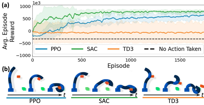
Fig. 4: Planar Block Pushing training results. (a) Reward history for the first 2000 training episodes for each algorithm. Curves are the average smoothed reward (window size 20) across three random seeds, and shaded regions indicate plus/minus one standard deviation. (b) Snapshots of policy rollouts over one episode representative of the best reliable behaviors developed by each algorithm. TD3 does not move the object (orange) all the way to the green goal position, while both PPO and SAC grasp and position the box successfully.
