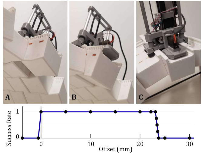
Fig. 7. The system is capable of self-correcting even large positioning errors. (A) When placing a block into the vault ~22 mm past its intended position, the insertion forces neighboring blocks out of its way. (B) After the RailBot retracts its gripper, the magnetic forces attempt to pull the block into alignment, but the robot’s body blocks its path. (C) The RailBot locomotes back toward the arch, allowing the block to settle in its intended position. (Below) The success rate when placing blocks an offset distance from the edge of the previous block in the row (0mm).
