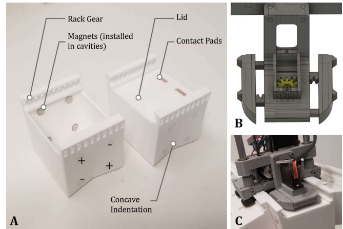
Fig. 3. (A) The blocks used in the demonstration measure roughly 50 mm \times 68 mm \times 57 mm and are 3D printed with embedded features like rack gears to facilitate robot locomotion, shaped faces to facilitate alignment and enhance structural stability, a channel to hold a lid, and cavities to mount magnets. Magnets are installed in a pattern of alternating polarity (the same pattern is mirrored on the reverse side). (B) Detail of the RailBot's gripper with the motor removed, showing the pairwise rack-and-pinion mechanism. (C) Detail of the robot's gripper, having just retracted after placing a block.
