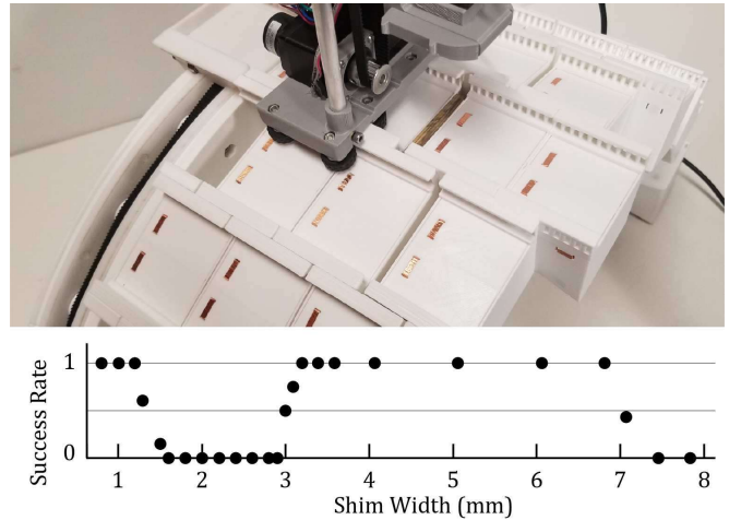
Fig. 6. Testing robustness to block misalignment by inserting a shim. Successively smaller gaps appear in adjacent rows. (Below) Gaps of 1.3–3.2 mm (~3–6% of block width) can disrupt locomotion.
