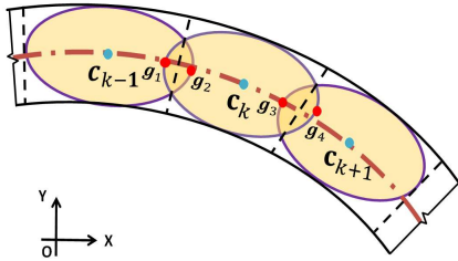
Fig. 4 Adjustment of the ellipses with overlaps.
