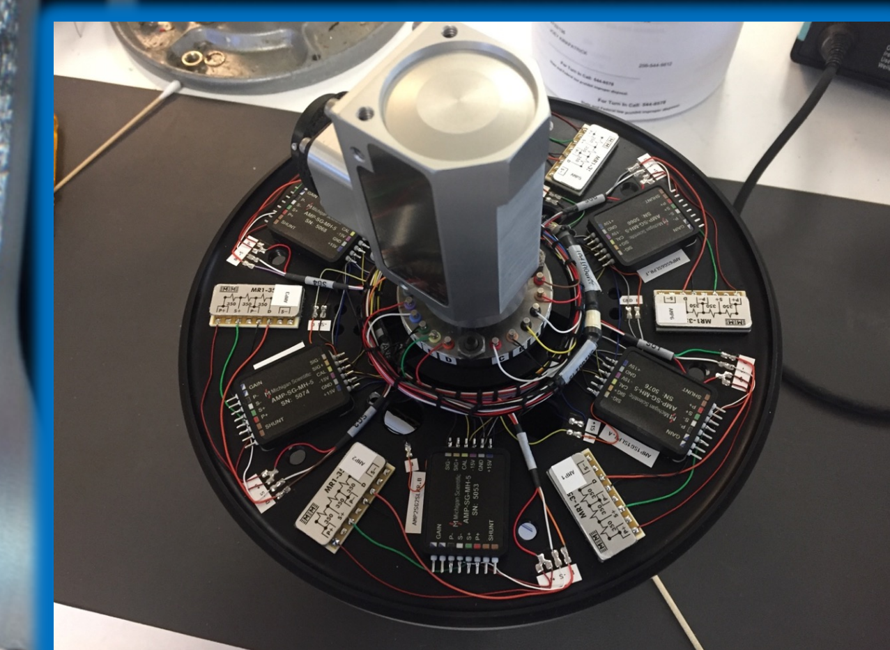
Slip Ring with On-Rotor Signal Conditioning
