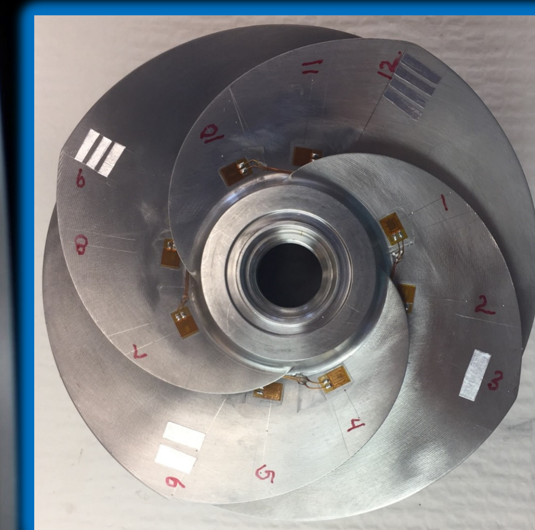
Strain Gauges Mounted on Inducer Blades
